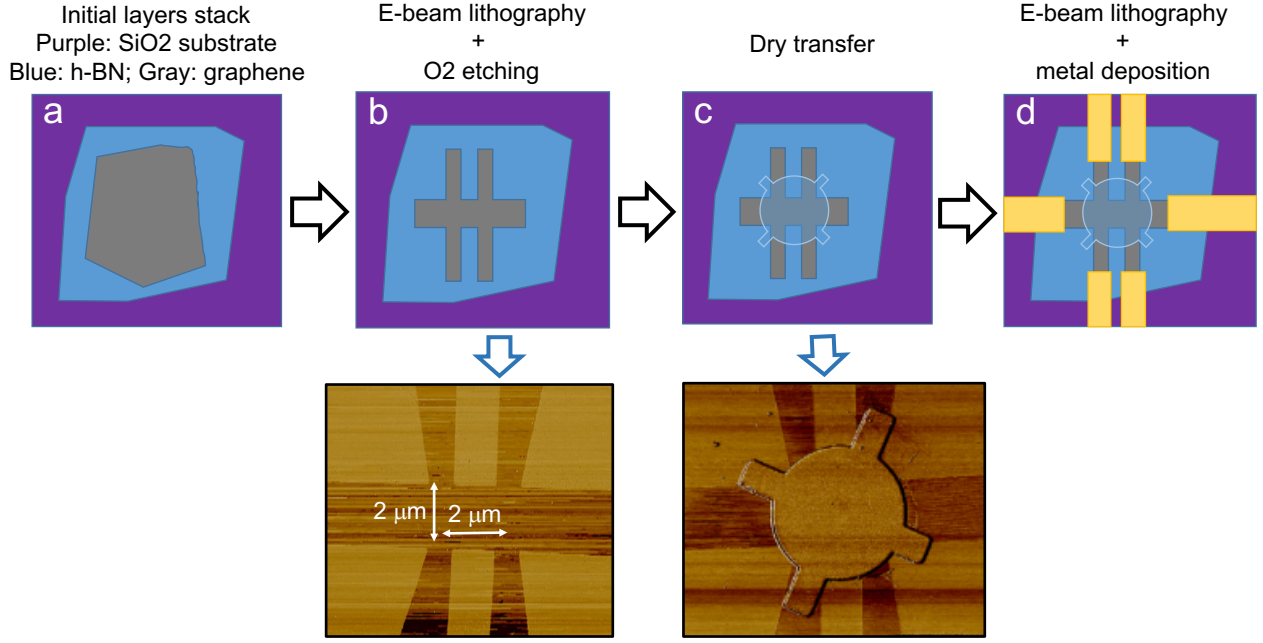
FIG. S1. Fabrication process. a , Initial graphene/BN stack deposited on a Si/SiO 2 substrate b , etching of the graphene flake to give a Hall bar shape. c , Dry transfer of a pre-shaped BN structure. d , electrical connection with Cr/Pd/Au top surface contacts.
