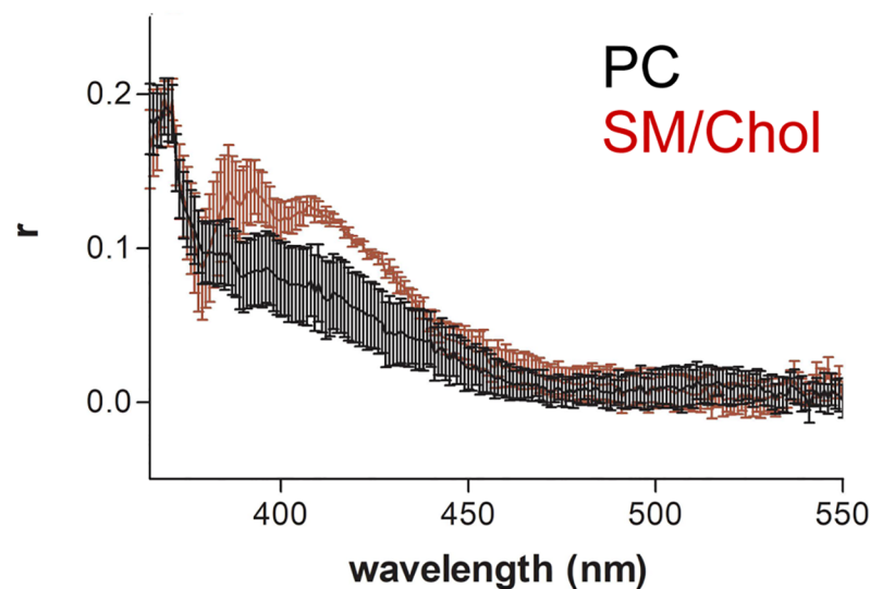
Fig 5. Fluorescence anisotropy (r) of Py-met-chol. LUVs were incubated at 35°C. Py-met-chol is at 3.6%, PC LUVs in black and SM/Chol in red. Curves are the mean \pm SEM of four independent experiments.
