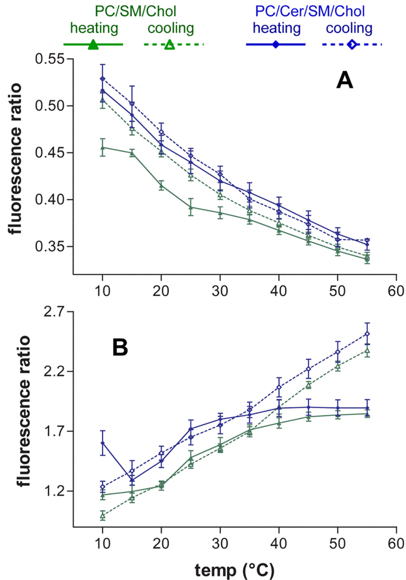
Fig 6. Ceramide effect on the evolution of Py-met-chole fluorescence in function of temperature. The probe concentration in LUVs is 3.6%. (A), cPyO3/cPyD9 ratio. (B), exci/iso ratio. Green lines ( \blacktriangle, \triangle ) PC/SM/Chol LUVs, blue lines ( \blacklozenge, \lozenge ) PC/SM/Cer/Chol LUVs. Continuous lines heating protocol and dotted lines cooling protocol. Means \pm SEM of 3 independent experiments.
