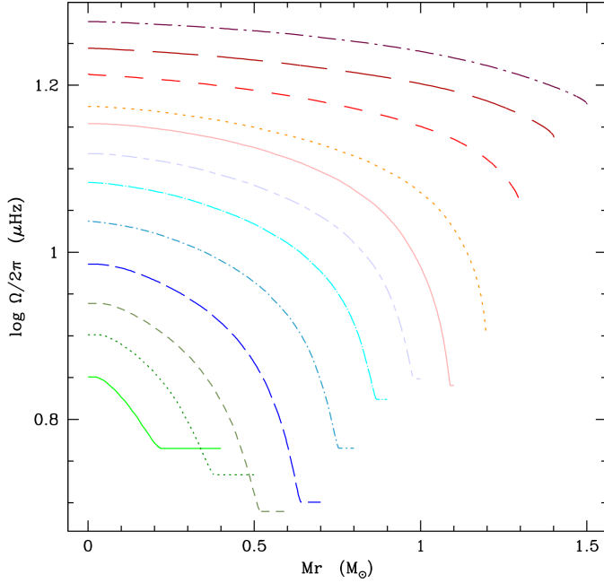
Fig. 9. Angular velocity profile as a function of the relative mass fraction of the median-rotating models at solar metallicity for the 0.4–1.5 M_{\odot} mass range on the ZAMS. The colour-coding is the same as in Fig. 6.
