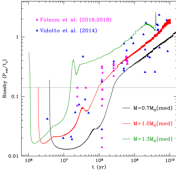
Fig. 13. Rossby number as a function of time for the 0.7 (black), 1.0 (red), and 1.3 (green) M_{\odot} models for median rotators. The Rossby number is estimated at half a pressure scale height above the base of the convective envelope. The dotted line indicates the saturation Rossby number at Ro = 0.14 . The blue and magenta triangles indicate the semi-empirical Rossby numbers for solar-like stars given in Folsom et al. (2016, 2018) and Vidotto et al. (2014b).
