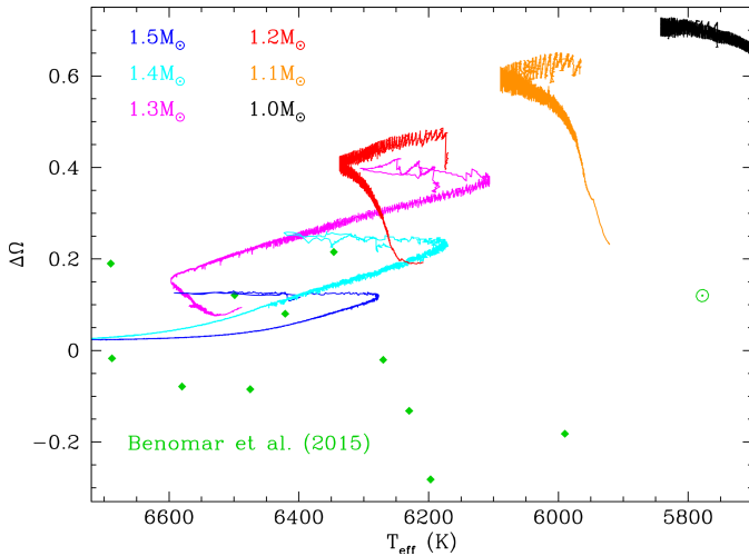
Fig. 10. Differential rotation ( \Delta\Omega ) as a function of effective temperature for our solar metallicity 1.0–1.5 M_{\odot} models with a median initial rotation rate. Green diamonds show the value of \Delta\Omega from the Benomar et al. (2015) data. The solar value as given by Fossat et al. (2017) is indicated by \odot .
