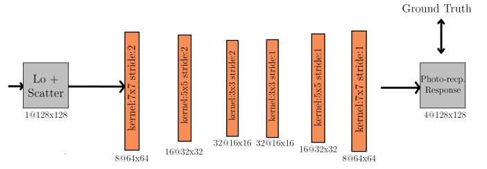
Fig. 3. Photo-receptor Spectral Sensitivity Neural Network box diagram.
