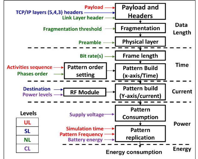
Figure 3. An energy-aware cross-level model for RF activities.
