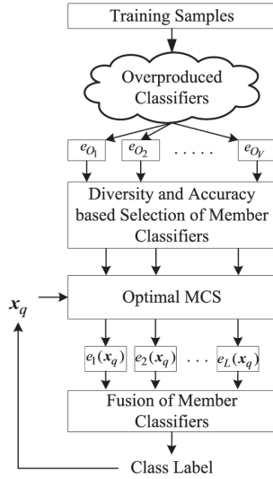
Fig. 3. Implementation of MCS based on diversity.
