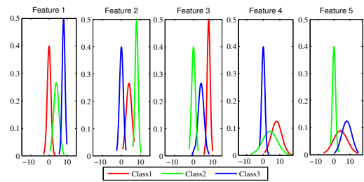
Fig. 5. 1-D artificial dataset.
