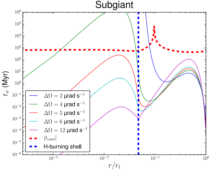
Fig. 1. Wave-driven timescale, Equation (3.1), as a function of the radius normalized by the radius at the top of the radiative zone, for a 1 M_{\odot} subgiant model. The contraction timescale and the location of the hydrogen-burning shell are represented by the red and blue dashed lines, respectively. Different amplitudes for \Delta\Omega are considered.
