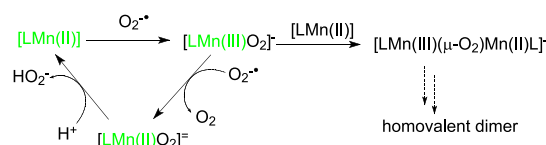
Scheme 2. Proposed Mechanism for the Reaction of 6 with KO_2
