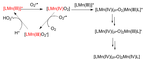
Scheme 1. Proposed Mechanism for the Reaction of 1–5 with KO_2
