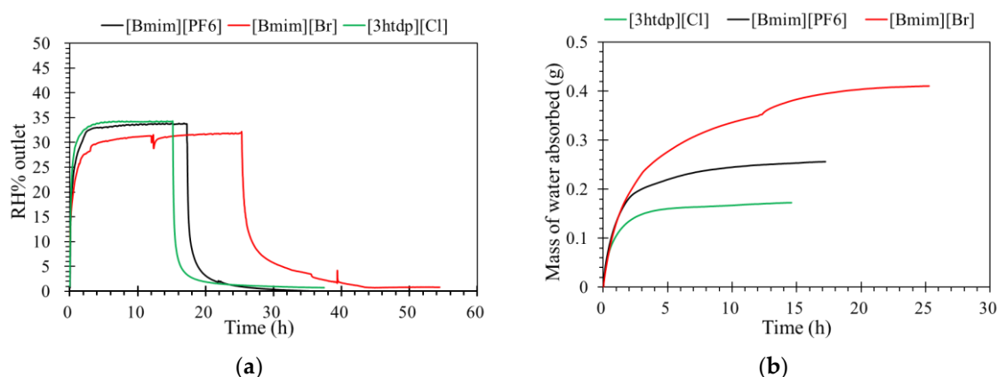
Figure 3. (a) The effect of ionic liquids filled into an ILM on its humidity separation performance; (b) the mass of water absorbed by an ILM with different ionic liquids. (relative humidity (RH)% inlet = 35%, temperature (T) = 32 °C, pressure = 1.0 atm, and flow rate = 0.5 L·min -1 ).
