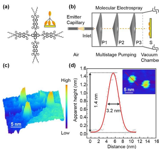
FIG. 1. (a) Chemical structure of the designed TP molecule, with the inset on the top-right showing the decoupling strategy. (b) Schematic of electro spray ionization for molecular deposition in vacuum. P1, P2, P3 shows differentially pumping stages and S represents the Au substrate. (c) A 3D view of STM topograph of single TP molecules on Au(111) (2.7 V, 2 pA, 27 \times 22 \text{ nm}^2 ). (d) Typical height profile of a single self-decoupled TP molecule on Au(111) for the line trace shown in the inset STM image (2.7 V, 2 pA, 20 \times 15 \text{ nm}^2 ).
