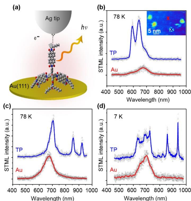
FIG. 3. (a) Schematic of STML setup for a single self-decoupled TP molecule on Au(111). (b) One example of STML spectra (2.7 V, 30 pA, 30 s) at 78 K measured at the labeled positions in the inset STM image (2.7 V, 2 pA, 33 \times 20 \text{ nm}^2 ). (c) Another example of STML spectra (2.7 V, 30 pA, 30 s) at 78 K. (d) One type of typical STML spectra (2.7 V, 2 pA, 300 s) acquired at 7 K. Solid lines show the smoothed curves with raw data denoted by the gray dots. The red curves are STML spectra measured on the bare Au(111) surface near TP molecules.
