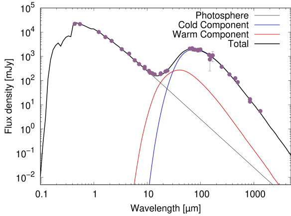
Figure 6. SED of 49 Cet using pure astronomical silicate with a bulk density of 3.3\text{g/cm}^3 for the outer and inner component. The thin black solid line represents the stellar photosphere, the red solid line shows the warm inner ring, the blue lines the outer belt.
