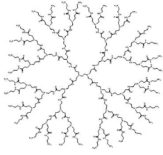
Biomedical dendrimers
