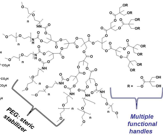
Polyester dendrimer-poly(ethylene oxide) bow-tie hybrids (Fréchet et al.)
