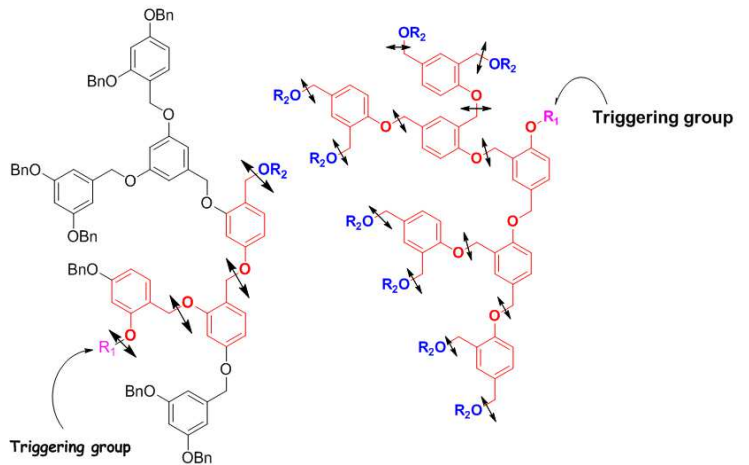
Self-immolative dendrimers (Fréchet et al., Shabat et al., Thonthwaite et al.)
