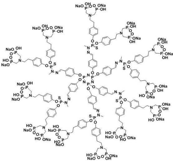
Azabis(dimethyl)phosphonate-based dendrimer (Caminade and Majoral et al.)
