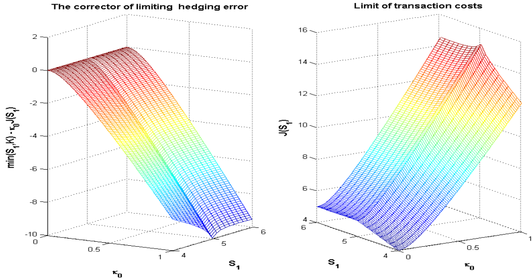
Figure 1: \min(S_1, K) - \kappa_* J(S_1) on the left and J(S_1) on the right with K = 5 .
