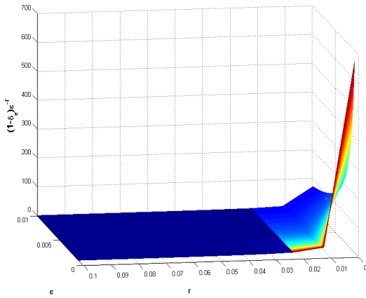
(a) Reduction factor 1 - \delta_\varepsilon and powers of \varepsilon
