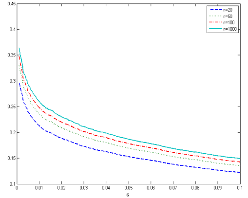
(b) Reduction amount and \varepsilon
