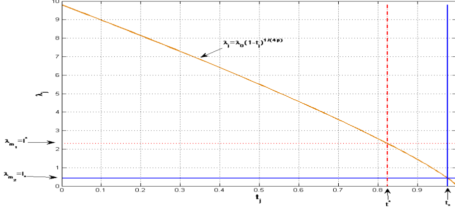
Figure 3: The sequences (\lambda_j) and (t_j) defined by (7.3).
