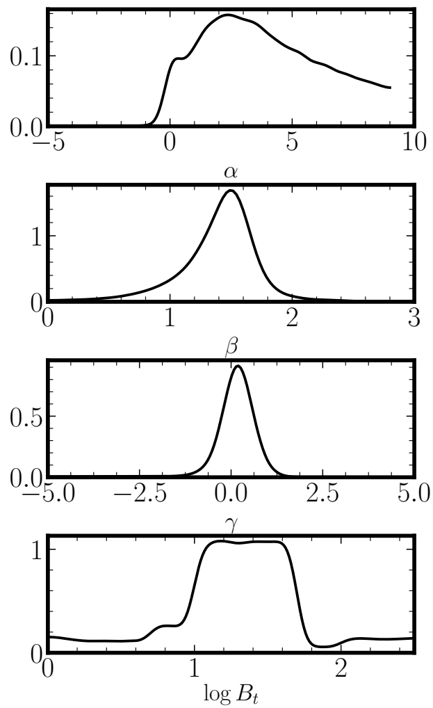
Figure 5: MCMC posterior distribution for the parameters of LR model B applied on MLT levels in rats
