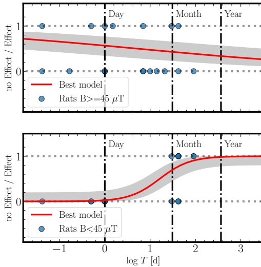
Figure 3: Bayesian Logistic Regression (model A) on rat studies with magnetic field strength B above (below) 45\mu T shown in the top (bottom) panel respectively
