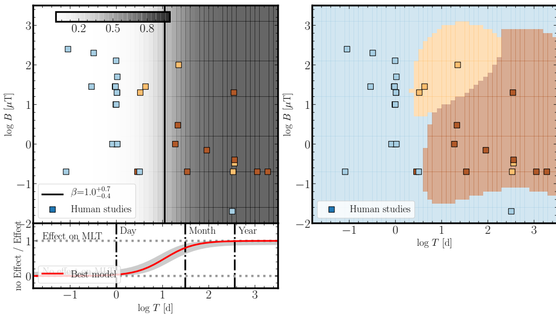
Figure 2: Left : Bayesian Logistic Regression (model A) on human studies. The top panel shows the data in the \log T - \log B plane along with the model A prediction (grey scale). The vertical line shows the best fit \beta parameter, i.e. where the probability p for having an effect is 0.5. The bottom panel shows the data as a function of exposure duration \log T and the red solid line represents the best fit logistic model with the shaded region representing the 95% posterior predictive interval. Right : Non-parametric Support Vector Classification (SVC) using a Radial Basis Function (RBF) kernel with penalty parameter C = 3.2 determined by cross-validation. In both panels, the x -values have been offsetted by a small (random) amount to help distinguish overlapping data points.
