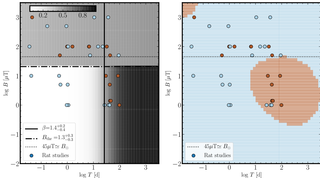
Figure 4: Left : Bayesian Logistic Regression (model B) on laboratory rat studies shown in the \log T - \log B plane shown along with the model predictions (grey scale). The horizontal dot-dashed line represents the best fit B_t threshold inferred by the model and the vertical solid line represents the best fit \beta parameter, i.e. where the probability p for having an effect is 0.5. Right : Non-parametric Support Vector Classification (SVC) using a RBF kernel with penalty parameter C = 3.2 determined by cross-validation. In both panels, the x -values have been offsetted by a small (random) amount to help distinguish overlapping data points.
