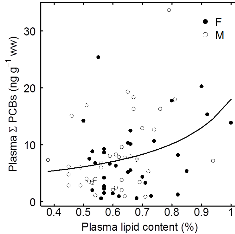
Fig. 2. PCBs concentrations increase with lipid content in blood of breeding wandering albatrosses from the Crozet Islands.
