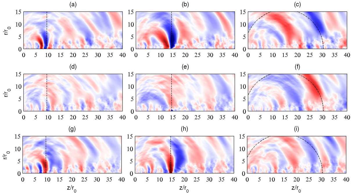
Fig. 8 Jet at \text{Re}_D = 100,000 . Correlations \mathcal{R} of (top) u'_z , (middle) |\omega|' and (bottom) p' at r = 0 and z = z_c with p'(r, z) for (left) \delta t = -8r_0/c_0 , (center) \delta t = 0 and (right) \delta t = 16r_0/c_0 , for n_\theta = 0 ; - - - positions for a downstream convection at 0.7u_j and a sound propagation at c_0 . The color scale ranges between \pm 0.25 , from blue to red.
