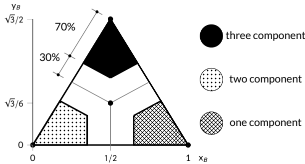
FIGURE 1 Definition of the anisotropy states in the barycentric map.
