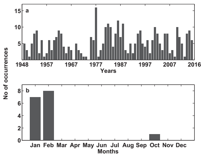
Figure 3. (a) Number of days in each year in which the sea level pressure instantaneous dimension extreme low ( d(z) ) state occurs (2% quantile; corresponding to the extreme Aleutian Low pattern). The maximum number of extremes occurred in 1977. (b) Number of extreme low sea level pressure instantaneous dimension ( d(z) ) occurrences per month in 1977.
