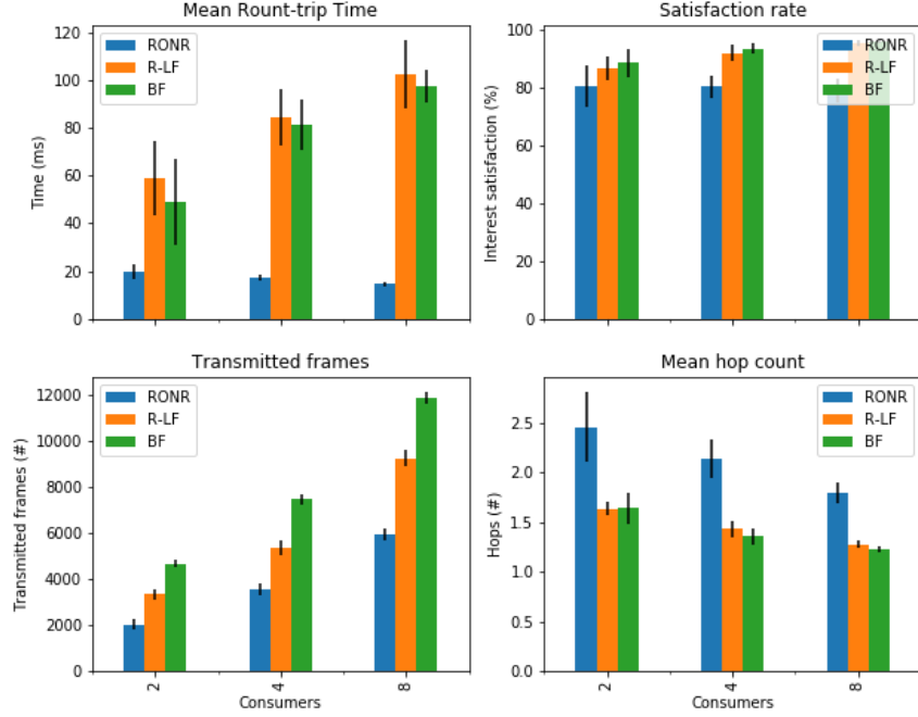
Figure 8: Multiple consumers and caching scenario results
