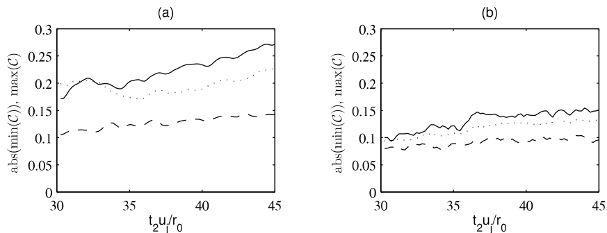
FIGURE 22. Representation of peak values of correlations between centerline quantities at t = t_1 and pressure fluctuations at r = 10r_0 at t = t_2 for (a) Re_D = 3,125 and (b) Re_D = 12,500 : — |\min(\mathcal{C}_{u'_z p'})| , - - - \max(\mathcal{C}_{u'_z u'_z p'}) , - · - · \max(\mathcal{C}_{|w|' p'}) , as a function of t_2 .
