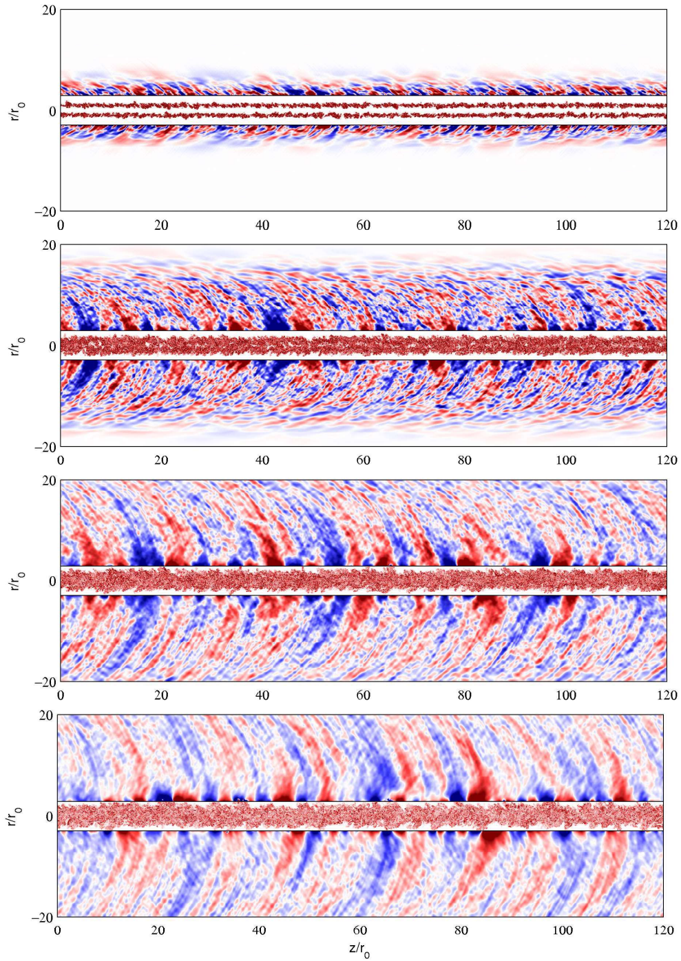
FIGURE 3. (Colour and movie online available at journals.cambridge.org/flm ) Representation of vorticity norm for r \leq 3r_0 and of pressure fluctuations otherwise, obtained for Re_D = 12,500 at t_{u_j}/r_0 = 10, 20, 30 and 40 , from top to bottom. The color scales range up to the level of 5u_j/r_0 for vorticity, and from -200 Pa to 200 Pa for pressure, from blue to red.
