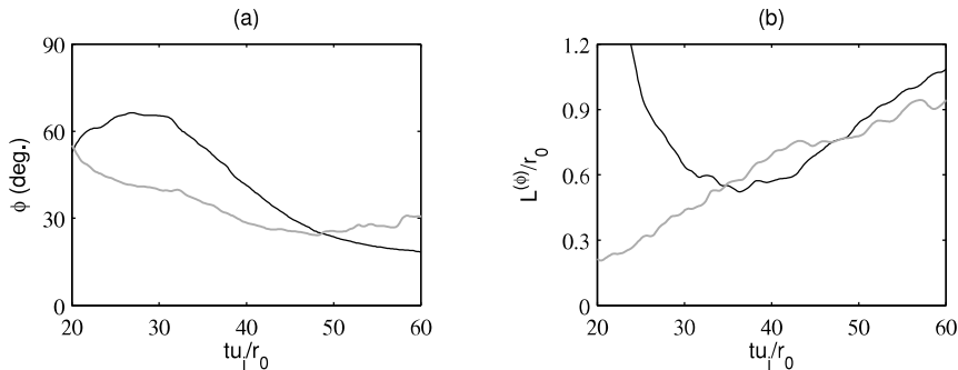
FIGURE 17. Time variations of (a) the radiation angle \phi and (b) the integral length scale L_\phi/r_0 along the average direction of acoustic propagation at r = 10r_0 for \text{Re}_D = 3,125 and \text{Re}_D = 12,500 .
