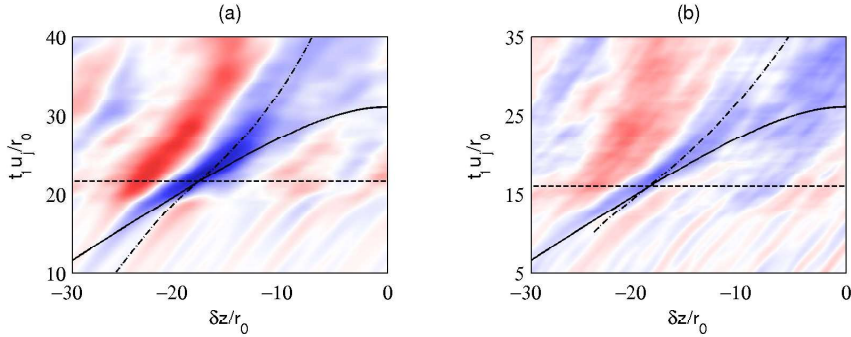
FIGURE 20. Space-time correlations C_{u'_z p'} obtained between velocity fluctuations at r = 0 and t = t_1 and pressure fluctuations at r = 10r_0 (a) at t_2 u_j / r_0 = 40 for Re_D = 3, 125 and (b) at t_2 u_j / r_0 = 35 for Re_D = 12, 500 . The color scale ranges from -0.30 to 0.30 , from blue to red; — propagation at the ambient speed of sound; - - - t_1 = t_c ; - · - · trajectory based on the convection velocity on the jet axis.
