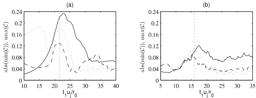
FIGURE 21. Representation of peak values of correlations between centerline quantities at t = t_1 and pressure fluctuations at r = 10r_0 (a) at t_2u_j/r_0 = 40 for Re_D = 3,125 and (b) at t_2u_j/r_0 = 35 for Re_D = 12,500 : — |\min(\mathcal{C}_{u'_z p'})| , - - - \max(\mathcal{C}_{u'_z u'_z p'}) , - · - · \max(\mathcal{C}_{|w|' p'}) , as a function of t_1 ; ···· t_1 = t_c .
