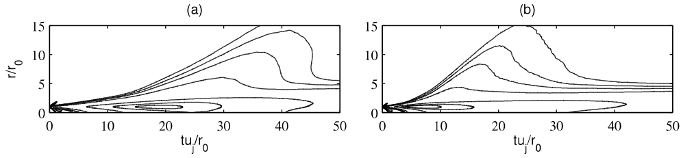
FIGURE 12. Space-time representation of the rms fields of pressure fluctuations for (a) Re_D = 3,125 and (b) Re_D = 12,500 using the contour line values \langle p'p' \rangle^{1/2} = 45, 60, 80, 140, 1000, 3000 and 5000 Pa.
