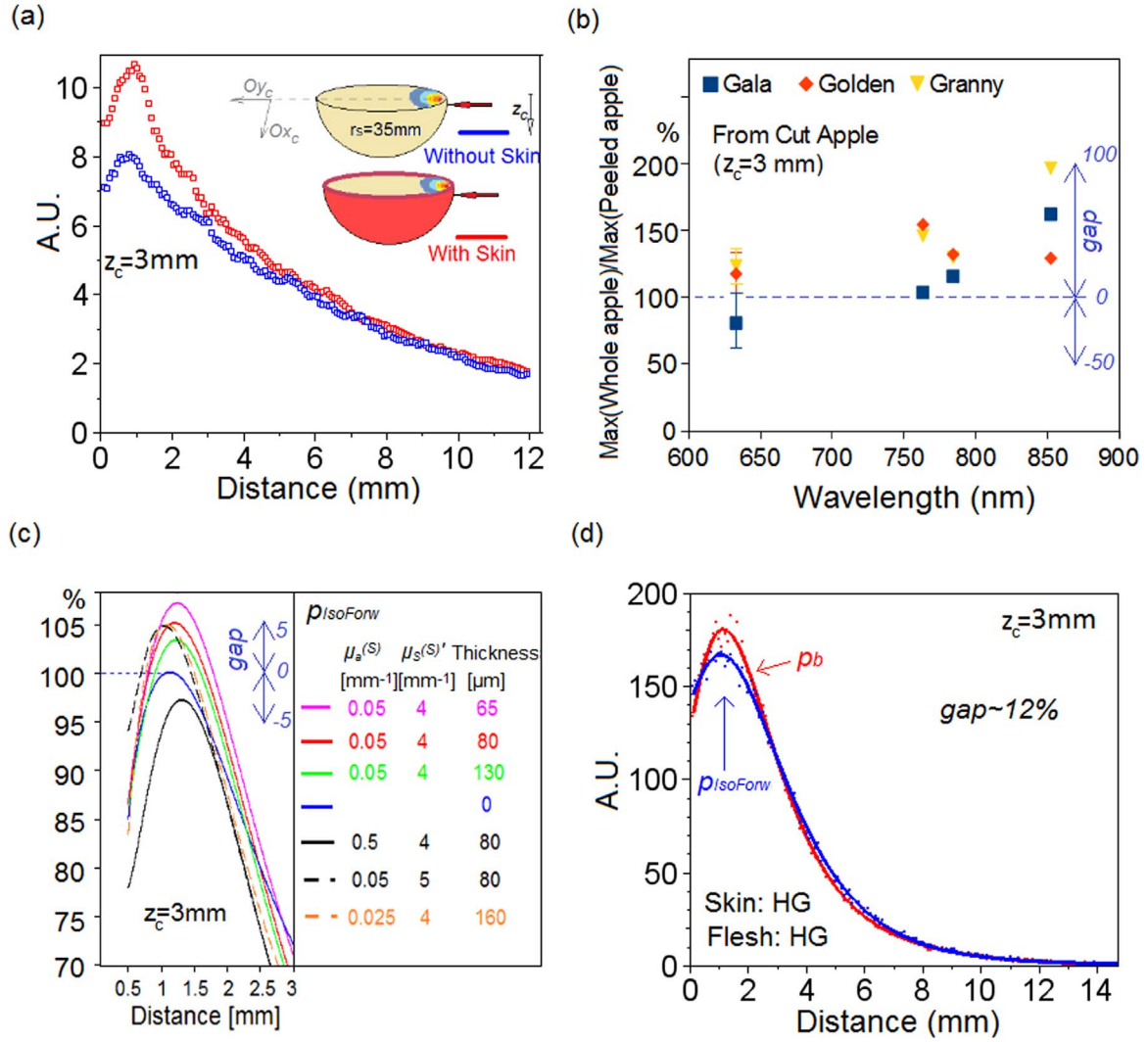
Fig. 6. Experimental averaged profiles, with skin (red) and without skin (blue), obtained in Transmittance mode at the surface of half-cut apples and z_c=3 mm. (a) Golden apple for 633 nm. (b) Ratio of peak intensities versus the wavelength. (c) Reflectance profiles extracted from simulation results with a neural network fitting (different skin layers, input p_{IsoForw}(z) ). (d) Simulated scattered light profiles where p_b(z) (Eq. (2)) and p_{IsoForw}(z) (Eq. (3)) are used for the unpeeled and peeled media, respectively. Flesh optical coefficients are identical to those used in Fig. 3. (For interpretation of the references to color in this figure legend, the reader is referred to the web version of this article).
