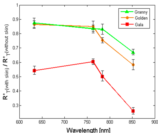
Figure 8. Plots of the total reflection ratio \alpha_R^* as a function of the wavelength, for three apple cultivars with and without skin.
