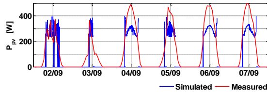
Fig. 8. Produced electrical power of PV-T collectors
