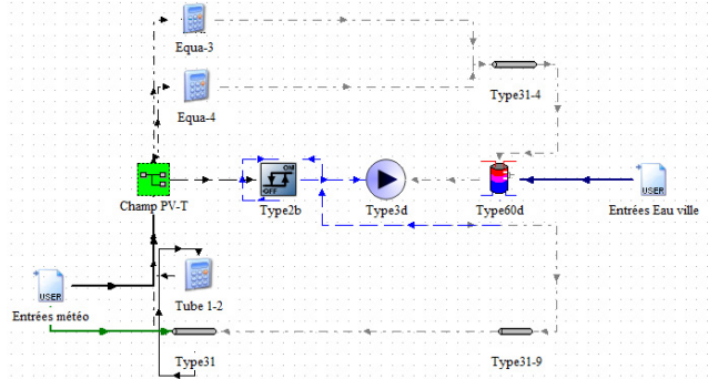
Fig. 3. TRNSYS model of a PV-T SDHW system
