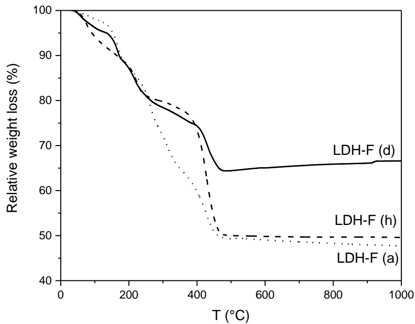
Figure S1: TGA of LDH-F powders under air (sample a, d and h)
