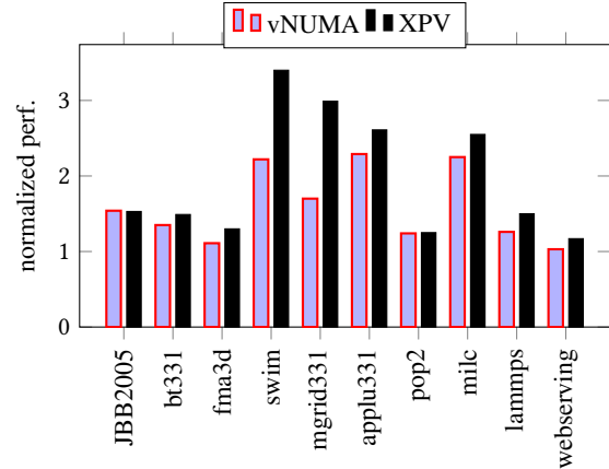
Figure 5. XPV implementation efficiency. XPV is compared with vNUMA (implementer by Xen) when no topology change occurs. The performance gap comes from the fact that the implementation of vNUMA by Xen is less optimized than XPV. Recall that the latter does not use any vNUMA code.
