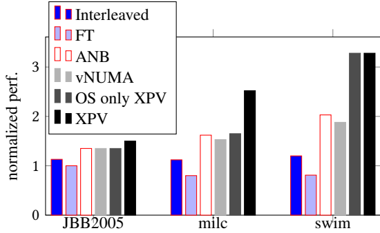
Figure 10. XPV facing memory ballooning (higher is better).
