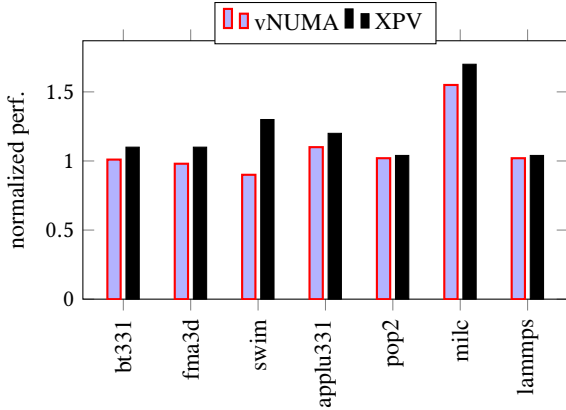
Figure 6. XPV implementation efficiency with small VMs.
