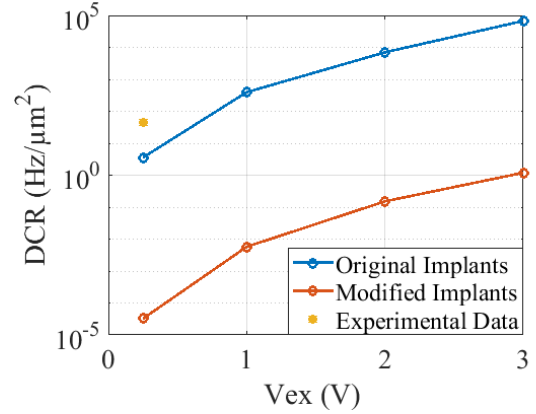
Figure 4. Simulated dark count rates (before and after)
