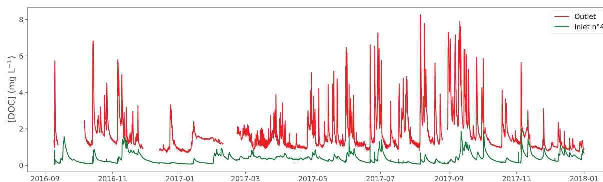
Figure 4. DOC concentration time series observed simultaneously at inlet 4 (green) and at the outlet (red) over 16 months (6 September 2016 to 31 December 2017).
