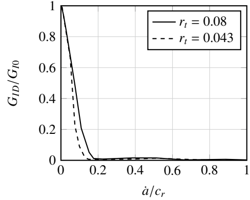
Fig. 7. Dynamic correction ratio for HSS regarding the crack velocity and the thickness.
