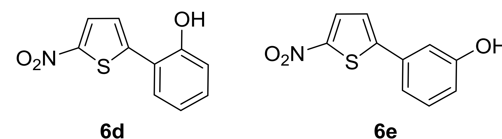
Figure 1: Structures of molecules 6d and 6e .
