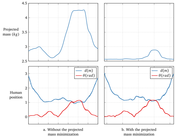
Fig. 2. Reconfiguration of the robot to minimize its perceived mass in the direction of a human. a. shows the projected mass for a given configuration of the robot when the human moves around it. b. shows the projected mass for the same human motion but with the active reconfiguration of the robot to minimize the projected mass.
