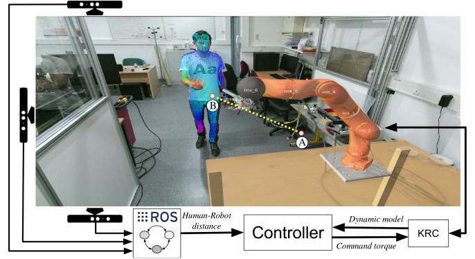
Fig. 1. Scene observed by the RGBD cameras (extracted from [8])
