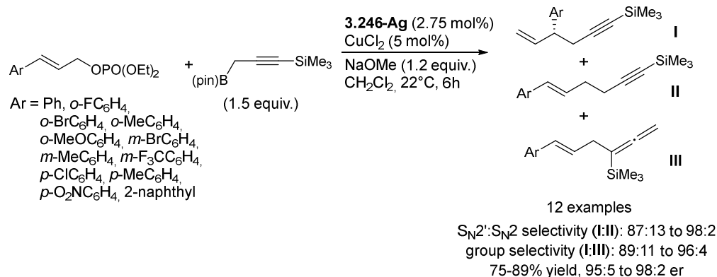
Scheme 3-34. Reaction of silyl-containing propargyl-B(pin) onto aryl-disubstituted allylic phosphates [171].
