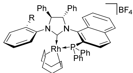
Chart 4-1. Rhodium complex described by Helmchen and coll. [185].
