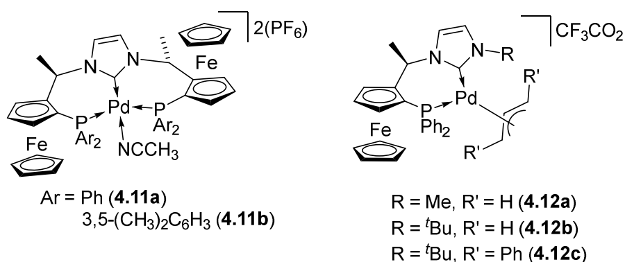
Chart 4-4. Palladium(II) complexes bearing tridentate ( 4.11 ) or bidentate ( 4.12 ) planar chiral ferrocenyl phosphine-NHC ligands [194,195,196].
