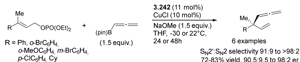
Scheme 3-33. Reaction of allenyl-B(pin) onto disubstituted or trisubstituted allylic phosphates [170].
