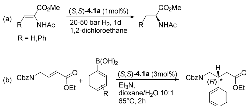
Scheme 4-1. (a) Asymmetric hydrogenation of N -acetamidoacrylate (R=H) or cinnamate (R=Ph); (b) Asymmetric conjugate addition of phenylboronic acid to an \alpha,\beta -unsaturated ester [187].
