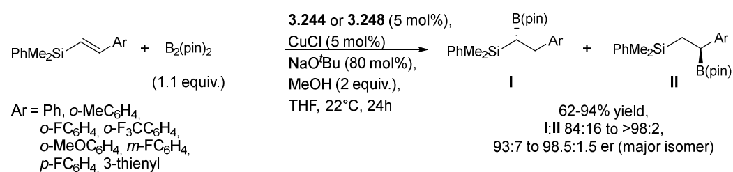
Scheme 3-40. Copper-catalyzed enantioselective synthesis of geminal borosilanes from aryl-substituted vinylsilanes [180].
