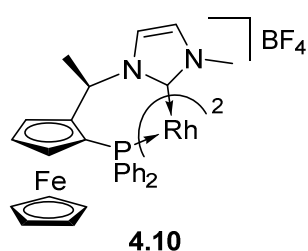
Chart 4-3. Rhodium(I) complex bearing planar chiral ferrocenyl phosphine-NHC ligands [193].
