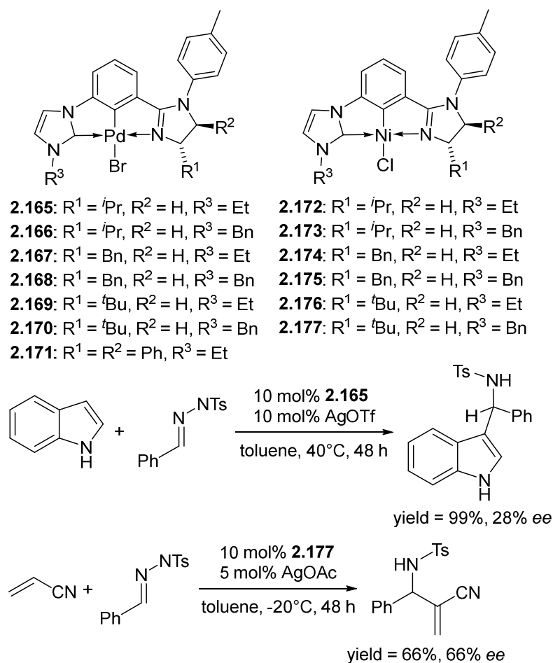
Scheme 2-21. Chiral N,C,C_{\text{NHC}} pincers developed by Zhu, Song et al. [83].
