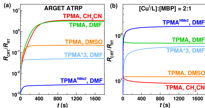
Figure 8. Ratio between the rate of CRT and RT in (a) ARGET ATRP of MA ([MA] = 5 M; [MA]:[MBP]:[Cu II Br 2 /L]:[Sn II ] = 250:1:0.05:0.25), and (b) reaction between 8×10 -3 M Cu I OTf/L and 4×10 -3 M MBP, with different catalysts and in different solvents, determined by PREDICI simulation (details on the simulations are presented in Figures S13-S27).
