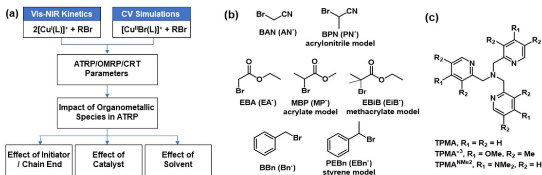
Scheme 2. (a) Workflow of determining the role of organometallic species in ATRP; (b) structures of investigated initiators (the terms in parentheses indicate the corresponding radicals after bromine transfer) and (c) structures of the investigated copper ligands.
