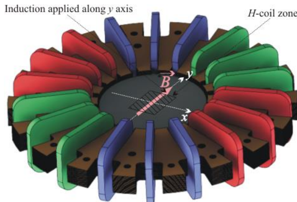
Fig. 12. An axis system x-y is defined on the sample surface. The three-phase currents are set in such a way that an alternating flux density of peak value B_p = 1.5 T is established along the y axis. The shadowed 20 mm square region centered on the sample surface is the H -coil zone.
