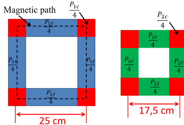
Fig. 3. Two Epstein frames with different limb lengths have been employed to determine the effective magnetic path length l_{eff}(J_p) . Its derivation relies on the assumption that the power loss in the corner regions is independent of the frame size [29][30].
