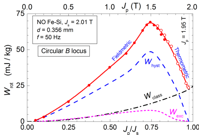
Fig. 22. Loss separation under rotating flux density up to J_p = 0.97J_s in a 0.356 thick NO Fe-Si sheet.
