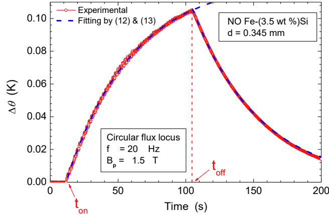
Fig. 17.: Temperature versus time in a non-oriented Fe-Si alloy subjected to rotational magnetic field strength at 20 Hz from time t_{on} to time t_{off} . The temperature difference \Delta\theta(t) follows an exponential dependence on time, with time constant \tau = c_p/K_{ext} , where c_p is the specific heat of the alloy and K_{ext} is the heat transmission coefficient, by which we lump the imperfect adiabatic response of the sample. The continuous fitting lines are calculated from (12) and (13).
