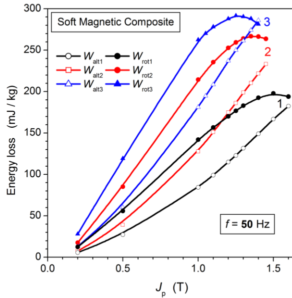
Fig. 20. Alternating W_{\text{alt}} and rotational W_{\text{rot}} energy loss measured at 50 Hz in three different types of Fe-based Soft Magnetic Composites. They are subjected to different preparation treatments, leading to different mass densities \delta . They attain the values: \delta_1 = 7450 \text{ kg/m}^3 , \delta_2 = 7260 \text{ kg/m}^3 , \delta_3 = 7110 \text{ kg/m}^3 .
