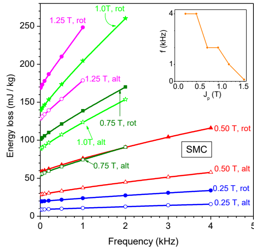
Fig. 19. Broadband energy loss under alternating and circular magnetic polarization measured with the high-frequency RSSM in a Soft Magnetic Composite. The curve shown in the inset roughly delimits the accessible (f, J_p) measuring domain.
