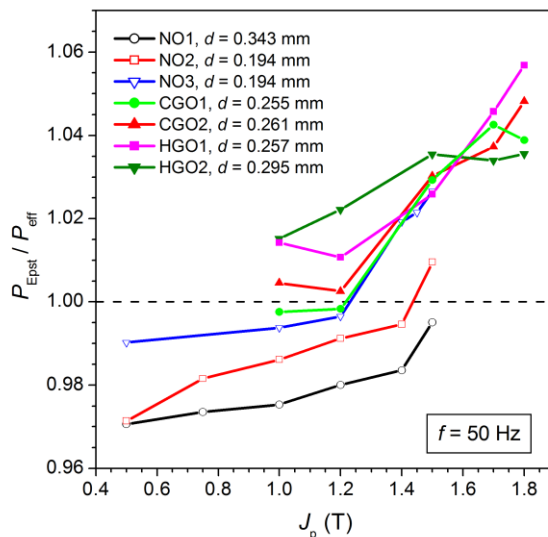
Fig. 1. Ratio of the Epstein to the effective (“true”) power loss figure P_{\text{Epsti}}/P_{\text{eff}} at 50 Hz measured in different types of non-oriented and grain-oriented steel sheets. P_{\text{eff}}(J_p) is obtained by precise local measurement of magnetic field strength and flux density.
