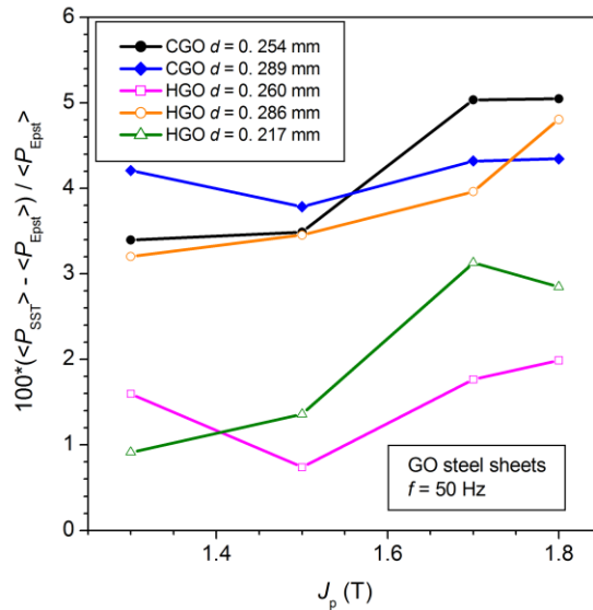
Fig. 5. The loss figure measured with the SST method P_{\text{SST}} (IEC60404-3) in CGO and HGO alloys is higher (~1 % - ~5 %) than the same quantity ( P_{\text{Epst}} ) measured using the Epstein frame (IEC60404-2) (adapted from [8], where the symbol \langle \cdot \rangle means the mean result between the different laboratories of the international comparison).
