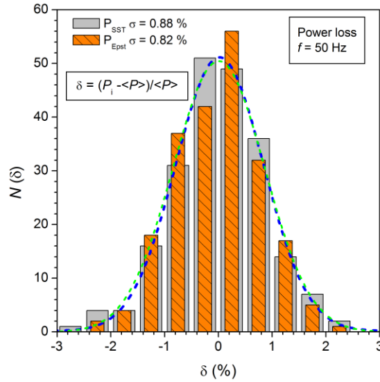
Fig. 2. Dispersion around the reference value of the laboratories best estimate of the power loss measured by the Epstein ( P_{Epst} ) and the SST ( P_{SST} ) methods in GO sheets. The related intercomparison is discussed in [8]. N(\delta) is the number of laboratories whose best estimate P_i deviates from the reference value \langle P \rangle by the relative quantity \delta = (P_i - \langle P \rangle) / \langle P \rangle . The dashed lines are best fits of the experimental distribution by a Gaussian function. The relative standard deviation \sigma associated with the measurements is lower than 1 %.
