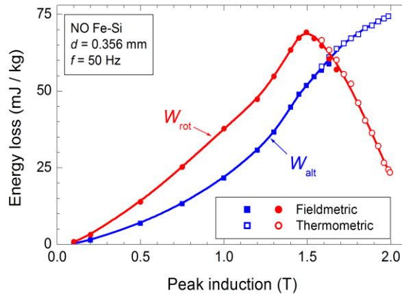
Fig. 21. Alternating W_{alt} and rotational W_{rot} energy losses in NO Fe-Si sheets measured at 50 Hz up to peak flux density B_p = 2.0 T ( J_p = 1.95 T).
