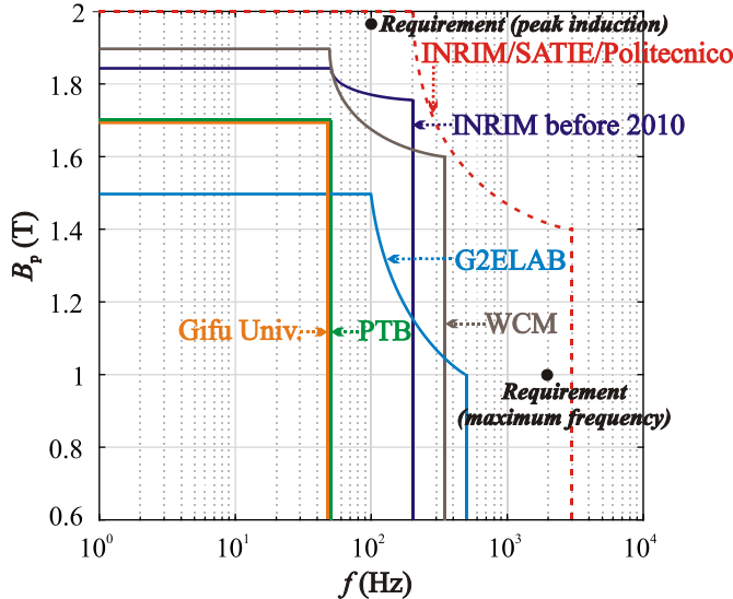
Fig. 10. Basic 2D measuring capabilities on non-oriented steel sheets by international laboratories are summarized in the B_p vs. frequency plane. The dashed line defines the enhanced upper limit jointly achieved by INRIM/SATIE/Politecnico di Torino.
