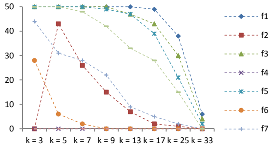
Figure 5: Success rates (50 runs). Regular graphs. Problem dimension D = 50 . Standard PSO with fixed-parameters.
