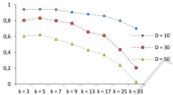
Figure 6: Percentage of successful runs averaged over the set of functions. Regular graphs. Fixed-parameters PSO.
