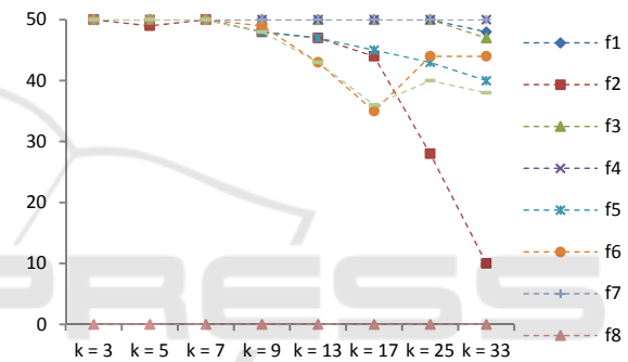
Figure 7: Success rates (50 runs). Regular graphs. Problem dimension D = 30 . PSO-TVAC.
