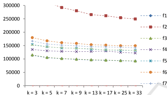
Figure 8: Evaluations required to meet criteria: median values (50 runs). Regular graphs. Problem dimension D = 30 . PSO-TVAC.
