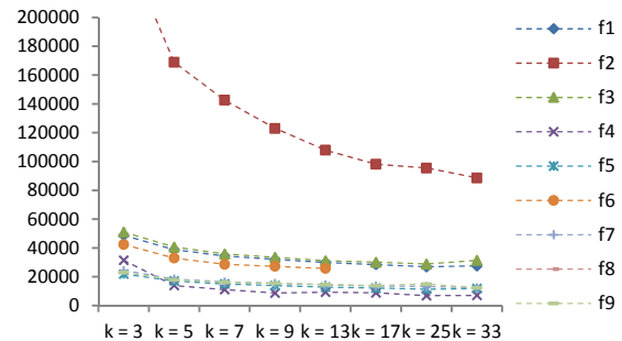
Figure 3: Evaluations required to meet criteria: median values (50 runs). Regular graphs. Problem dimension D = 30 . Fixed-parameters PSO.
