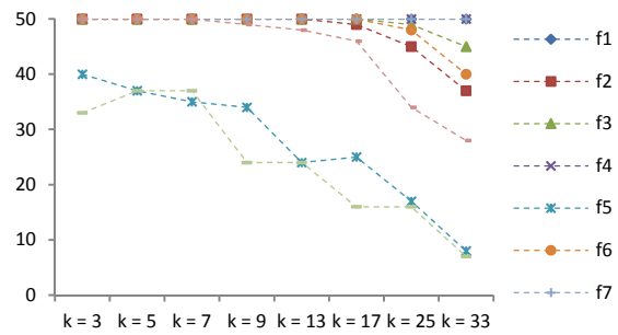
Figure 4: Success rates (50 runs). Regular graphs. Problem dimension D = 10 . Standard PSO with fixed-parameters.
