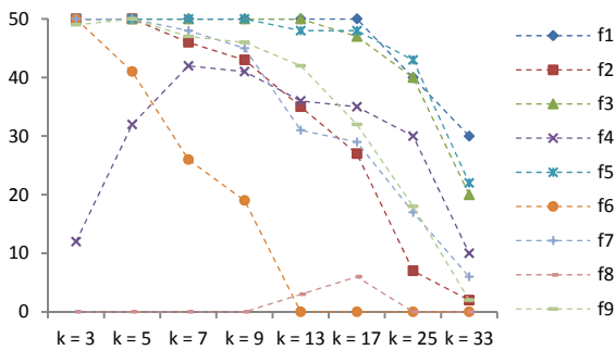
Figure 2: Success rates (50 runs). Regular graphs. Problem dimension D = 30 . Standard PSO with fixed-parameters.
