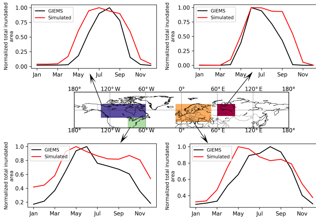
Figure 6. Simulated and observed (GIEMS; Prigent et al., 2007, 2012) mean seasonality (averaged over 1993–2007) of total inundated area. Note that the simulated and observed total inundated areas of each month are divided by the simulated and observed maximum monthly values, respectively, to highlight seasonality of inundation rather than comparing absolute values of inundated area.
