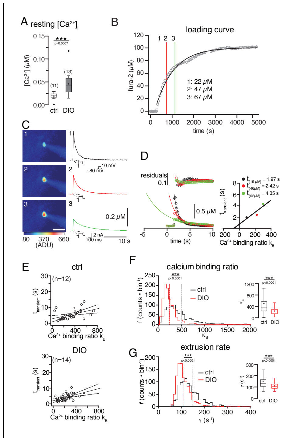
Figure 3. Diet-induced obesity changes the endogenous \text{Ca}^{2+} -handling properties of POMC neurons. \text{Ca}^{2+} handling was analyzed using a combination of patch-clamp recordings, ratiometric \text{Ca}^{2+} imaging, and the ‘added buffer approach’. (A) \text{Ca}^{2+} resting level. The concentration of free cytosolic \text{Ca}^{2+} was increased in DIO mice. (B–G) \text{Ca}^{2+} -handling properties. (B) fura-2 loading curve. POMC neurons were loaded via the patch pipette with the ratiometric \text{Ca}^{2+} indicator fura-2, which also serves as the added \text{Ca}^{2+} buffer. Fura-2 fluorescence was acquired at 360 nm excitation (isosbestic point of fura-2) every 30 s, and converted into fura-2 concentrations. (C) Decay kinetics of voltage-induced \text{Ca}^{2+} transients of the POMC neuron in (B). The images (left panels) were acquired at times indicated in (B) and demonstrate the increasing fura-2 concentration during loading. The graphs (right panels) demonstrate the effect of increasing added \text{Ca}^{2+} buffer (fura-2) concentrations on the decay kinetics of voltage-evoked \text{Ca}^{2+} transients. (C and D) Analysis of endogenous \text{Ca}^{2+} -handling parameters in a single cell. With Figure 3 continued on next page
