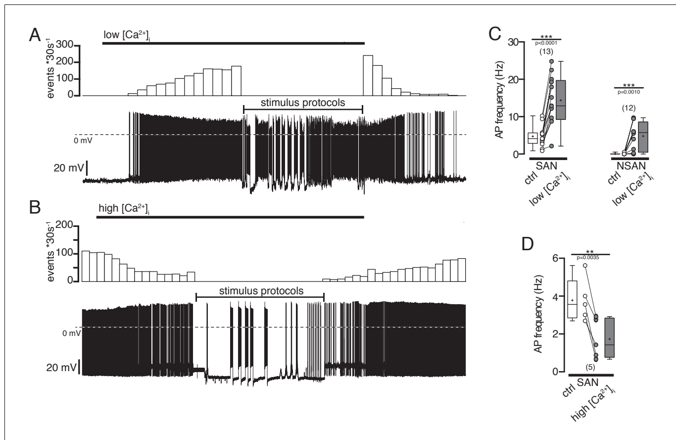
Figure 6. Effect of intracellular \text{Ca}^{2+} concentrations on action potential frequency of POMC neurons. (A and B) Original recordings of POMC neurons illustrating the effect of decreasing or increasing intracellular \text{Ca}^{2+} concentrations. (A) A silent POMC neurons started to generate action potentials with decreasing [\text{Ca}^{2+}]_i . The effect reverted to control levels at normal [\text{Ca}^{2+}]_i . (B) In a spontaneously active neuron, the AP frequency was reduced with increasing [\text{Ca}^{2+}]_i . The effect reversed at normal \text{Ca}^{2+} levels. (C) Action potential frequency of spontaneously active and silent POMC neurons at normal and low [\text{Ca}^{2+}]_i , respectively (paired t-test). (D) Action potential frequency of spontaneously active neurons at normal and high [\text{Ca}^{2+}]_i , respectively (paired t-test). SAN, spontaneously active neuron; NSAN, not spontaneously active neuron ( F < 0.5 Hz). ** p < 0.01 , *** p < 0.001 .
