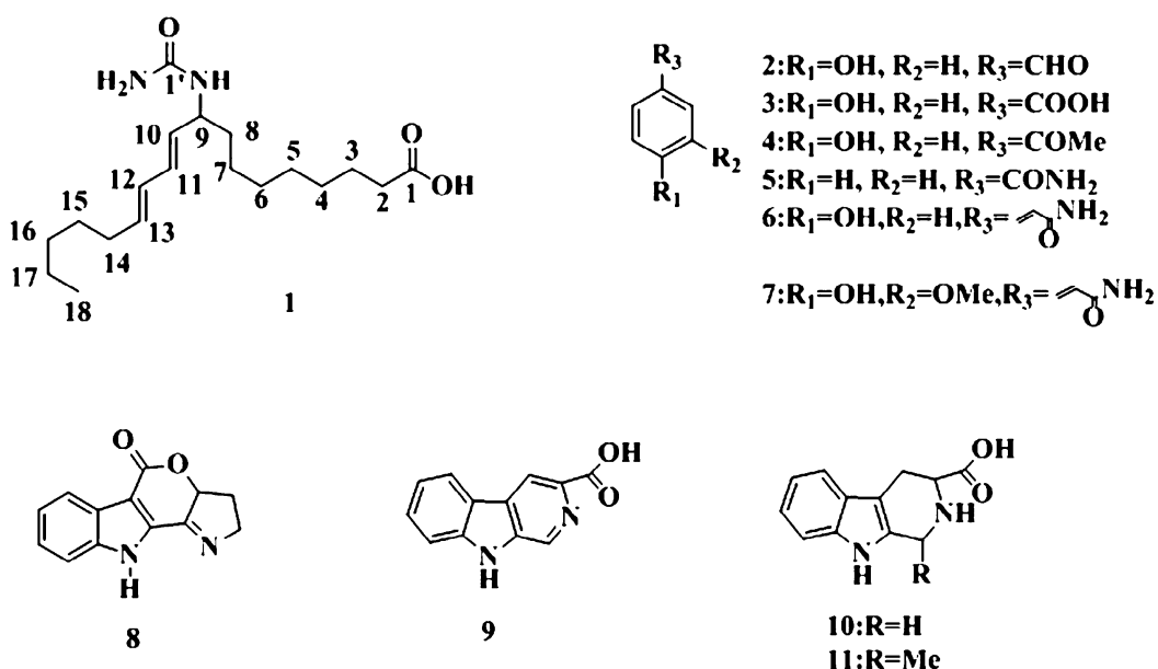
Figure 1. Chemical structures of compounds isolated from P. oleracea
