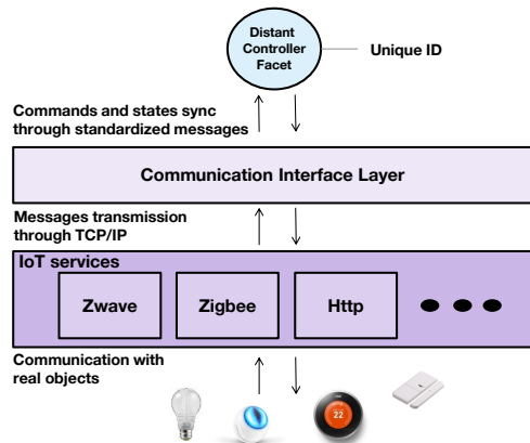
Figure 3: Distant Controller facets communicate with real objects thanks to a communication layer that is interfaced with IoT hardware services. Each real object is configured with a unique id.
