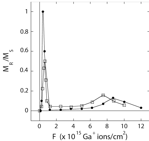
Fig. 3. Variation of the normalized remnant magnetization with the Ga + ion fluence for the uniformly irradiated (●) or FIB irradiated (□) Pt/Co(3 nm)/Pt sputtered film. The lines are guides for the eyes.
