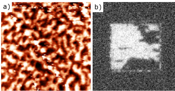
Fig. 10. ac-demagnetized states in quasi-uniformly FIB irradiated areas in the Pt/Co(3 nm)/Pt sputtered film. (a) MFM image ( 10 \times 10 \mu\text{m}^2 ) for F = 5 \times 10^{14} \text{Ga}^+ ions/ \text{cm}^2 ; (b) PKR image of a central square area ( 10 \times 10 \mu\text{m}^2 ) irradiated with F = 7.7 \times 10^{15} \text{Ga}^+ ions/ \text{cm}^2 . Large remnant domains with up and down magnetization can be visualized.
