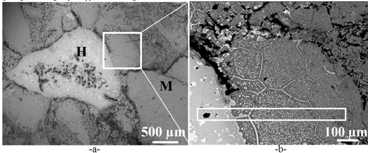
Figure 7: SEM micrograph highlighting a) a hercynite aggregate and b) the diffusion zone around hercynite
