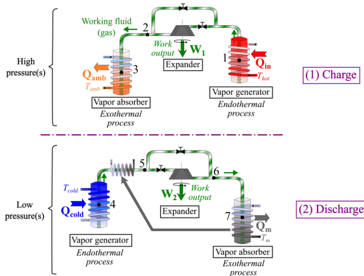
Figure 1. Working principle of hybrid thermochemical cycles: components, mass and energy flows in each step of operation (Charge / Discharge).
