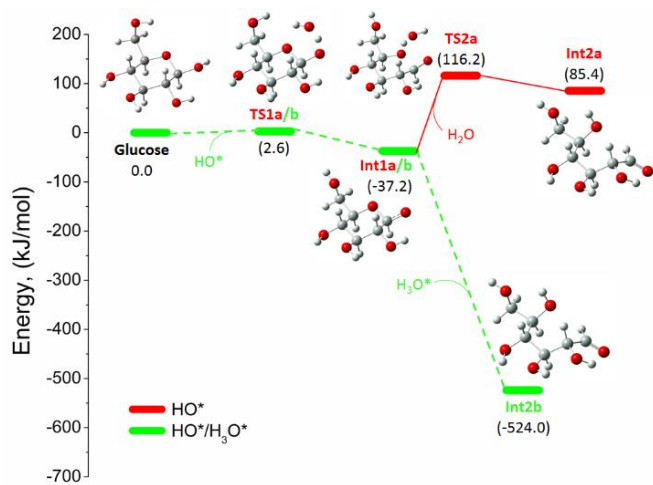
Figure 1. Potential energy profiles for glucose ring-opening reaction in vacuum calculated at the \text{Mo5-2X/6-311+G(d,p)} level of theory facilitated by \text{HO}^\bullet , \text{HO}^\bullet/\text{H}_3\text{O}^\bullet radicals ( \text{H}^\bullet + \text{H}_2\text{O} ). Label of structure: Int : intermediate compounds; TS : transition state.
