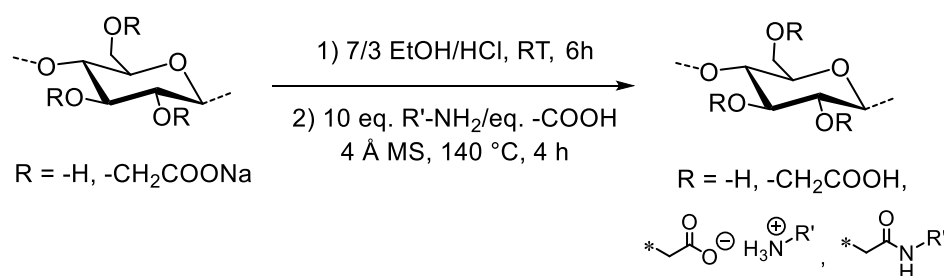
Scheme 1. Experimental conditions used for thermal amidation of carboxymethyl cellulose (CMC).
