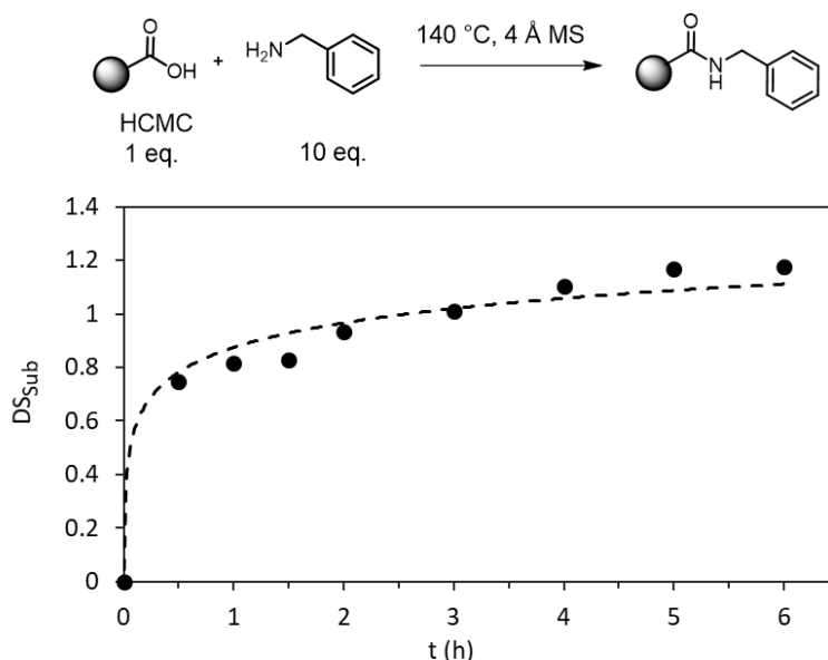
Figure 6. Evolution of \text{DS}_{\text{Sub}} with time for the reaction between HCMC and benzylamine. The dotted line serves as a guide to the eye.
