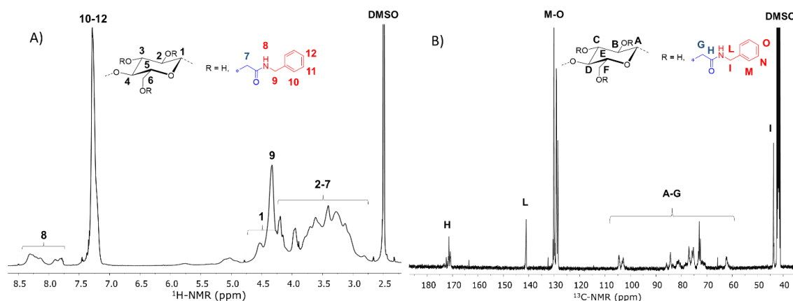
Figure 4. 1 H- (A) and 13 C-NMR (B) of CMC-Benz (Table 1, Entry 3), in DMSO-d 6 and at 358 K.
