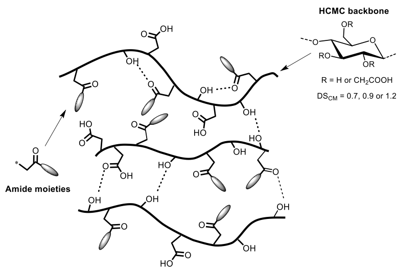
Figure 8. Schematic structure of internally plasticized CMC derivatives.
