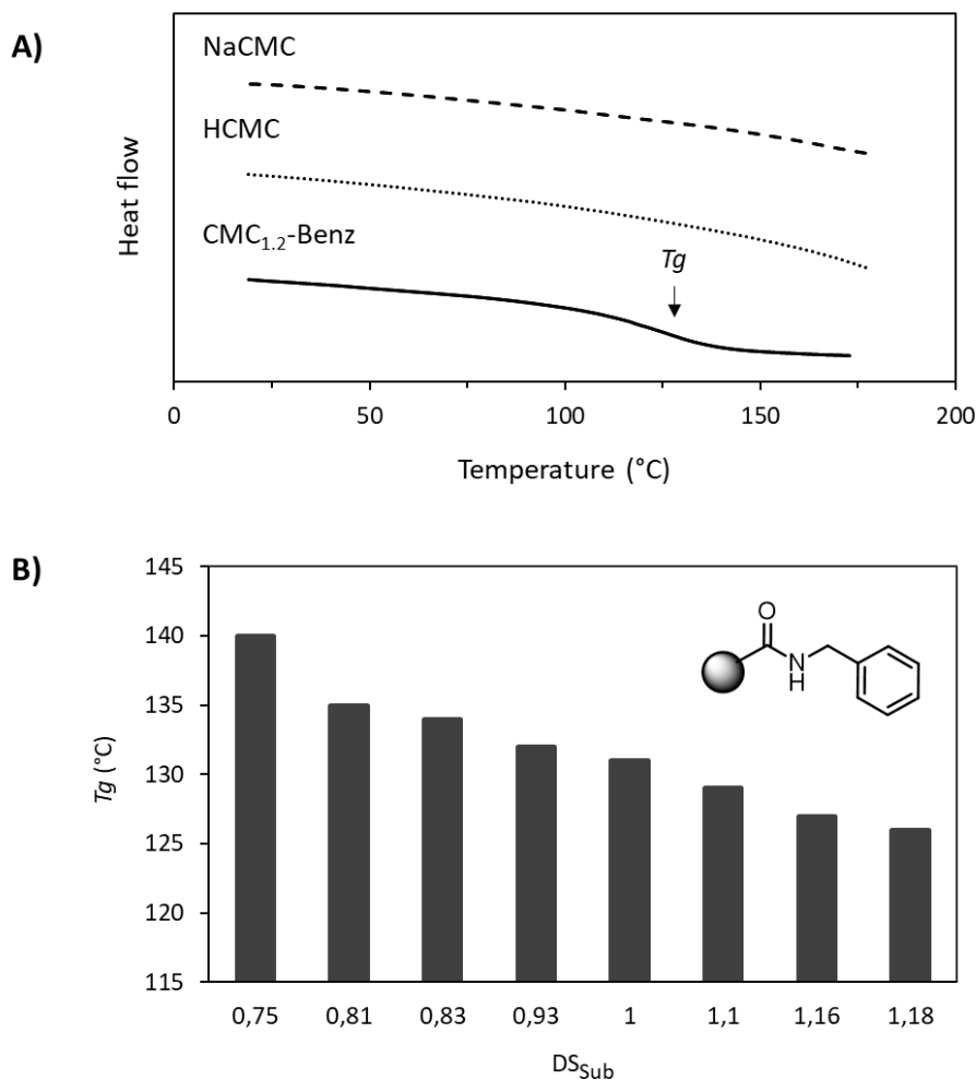
Figure 9. (A) Differential scanning calorimetry (DSC) curves of NaCMC, HCMC and CMC 1.2 -Benz (Table 1, Entry 3); (B) Evolution of T g values of the amidated CMC-Benz derivatives as a function of DS Sub .
