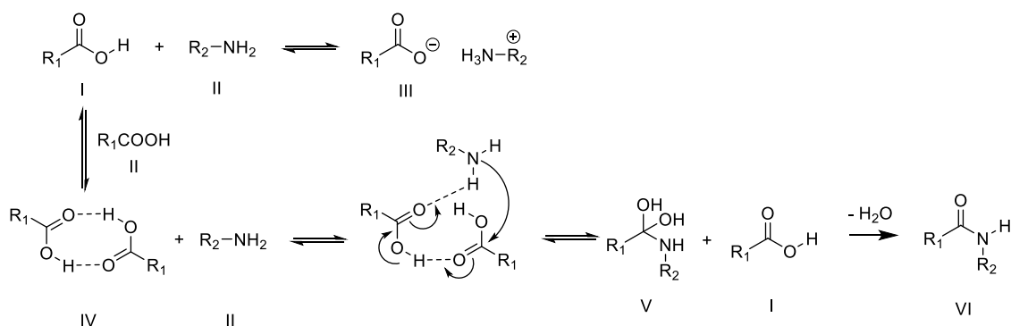
Figure 1. Mechanism of the thermal amidation of carboxylic acids.
