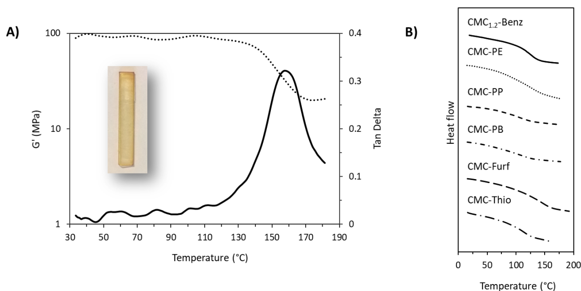
Figure 10. (A) Evolution of moduli G' (---) and of the loss tangent ( \tan \delta ) (—) as a function of temperature for a film made from \text{CMC}_{1,2}\text{-Benz} (Table 1, Entry 3); (B) DSC curves of \text{CMC}_{1,2}\text{-Benz} (Table 1, Entry 3), \text{CMC-PE} (Table 1, Entry 6), \text{CMC-PP} (Table 1, Entry 7), \text{CMC-PB} (Table 1, Entry 8), \text{CMC-Furf} (Table 1, Entry 11), \text{CMC-Thio} (Table 1, Entry 12).
