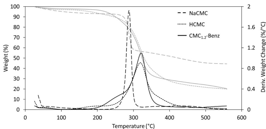
Figure 7. Thermogravimetric analysis (TGA) curves of NaCMC and CMC_{1,2} -Benz (Table 1, Entry 3): Weight (%), grey lines, and Derivative Weight Change (%/°C), black lines.
