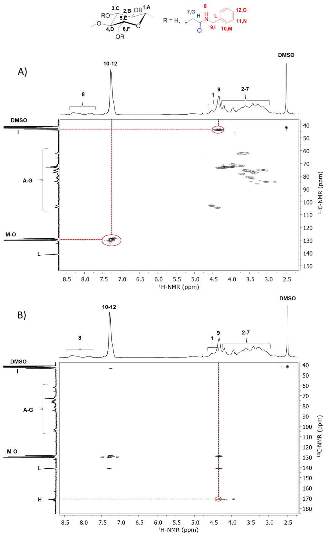
Figure 5. Heteronuclear Single-Quantum Correlation (HSQC) (A) and Heteronuclear Single-Quantum Correlation (HMBC) (B) spectra of product CMC-Benz (Table 1, Entry 3), in DMSO-d 6 and at 358 K.
