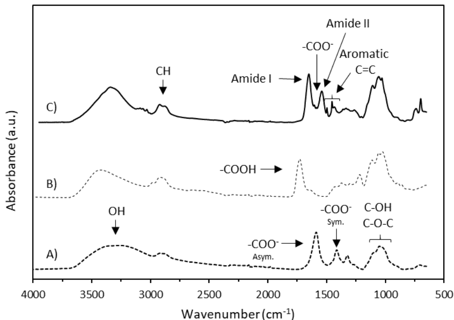
Figure 3. FT-IR of NaCMC (A,-----), HCMC (B,.....) and CMC 1,2 -Benz (Table 1, Entry 3) (C,—).
