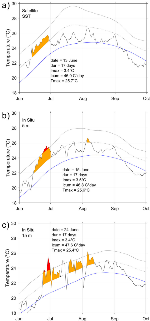
Figure 4.4.5. Information on MHW events in Scandola Marine Protected Area nearshore waters (Parc Régional de Corse, France). (a–c) Time series of daily satellite sea surface temperature and in situ temperature measured at 5 and 15 m depth. Climatology (blue line) and MHW thresholds (grey lines) calculated over the period 2004–2016 are also shown. MHW events are identified and filled with colours by categories (orange = moderate, red = strong). (d) In situ temperature anomalies relative to the multi-year mean at 10, 25 and 40 m depth. (e) Total number of MHW days from satellite (0 m) and in situ data (5–40 m depth). Reference number of the products used: 4.4.1 and 4.4.2.
