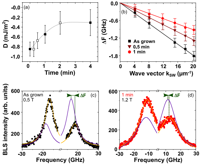
FIG. 3: (a) DMI constant D as a function of the biasing time, values calculated using estimated M_s values are shown as empty symbols. The dotted line is a guide to the eye. (b) Frequency asymmetry as a function of the wave vector and linear fitting lines. BLS spectra at k_{SW} = 20 \mu m^{-1} for the (c) as-grown and (d) 1 minute biased films. The solid lines correspond to the Lorentzian fitting.
