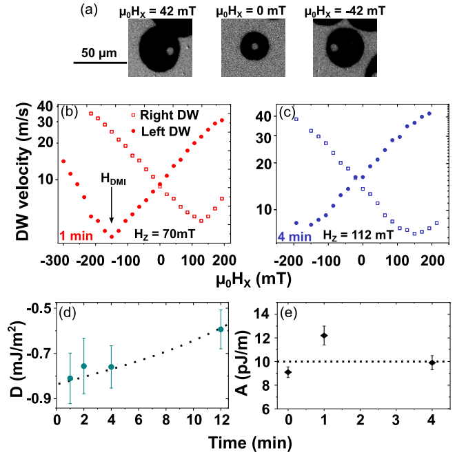
FIG. 4: (a) Kerr microscopy images of the domain expansion in the sample biased for 1 minute under in-plane fields ( \mu_0 H_X ). Velocity curves as a function of \mu_0 H_X from films biased for 1 (b) and 4 (c) minutes, respectively. (d) DMI parameter D extracted using the experimentally obtained values of A shown in (e). Lines are a guide to the eye.
