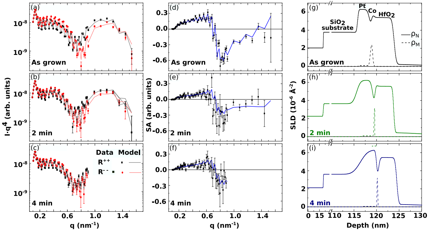
FIG. 7: (a-c) PNR signals R^{++} and R^{--} as a function of the wave vector and the corresponding fitting lines, the spin asymmetry is plotted in (d-f). The scattering length density (SLD), the model used to fit the experimental data, is presented in (g-i).
