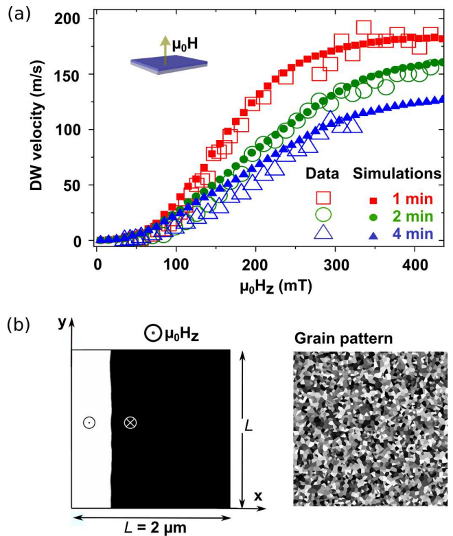
FIG. 5: (a) Experimental domain wall velocity as a function of a perpendicular magnetic field for films biased for 1 minute, 2 minutes and 4 minutes (empty symbols) and micromagnetic simulations (full symbols). (b) Granular structure used for the micromagnetic simulations.
