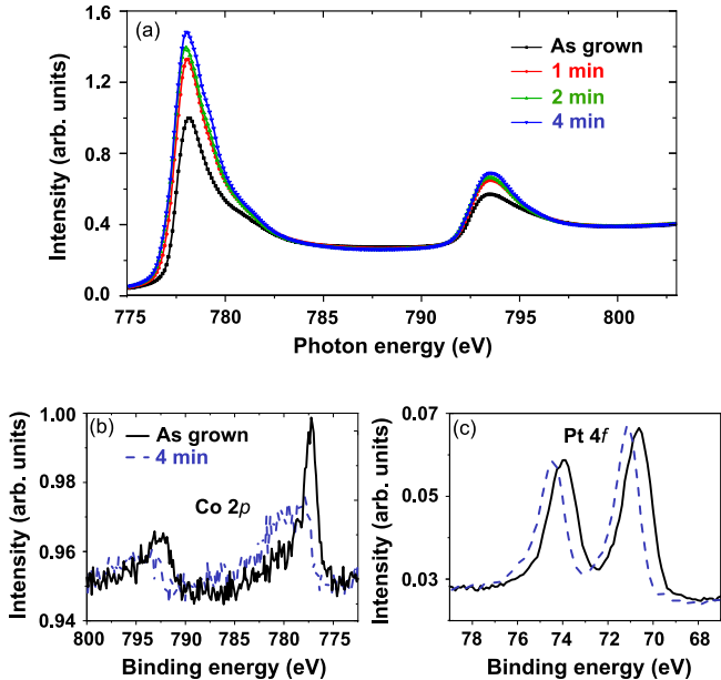
FIG. 6: (a) XAS spectra at the Co L_2 and L_3 edges as a function of the biasing time. XPS spectra at the (b) Co 2p_{3/2} and (c) Pt 4f regions for an as-grown sample (solid lines) and a sample biased for 4 minutes (dotted lines).
