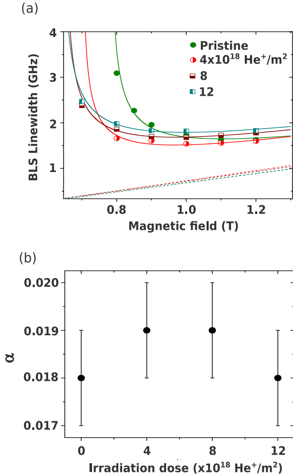
FIG. 7: BLS linewidth as a function of the applied in-plane magnetic field, solid lines going through the datapoints correspond to a fitting using Eq. (2) while the lines at the bottom of the graph are simulated neglecting the inhomogeneous contribution to the effective damping. (b) Gilbert damping parameter extracted from the fittings in (a).
