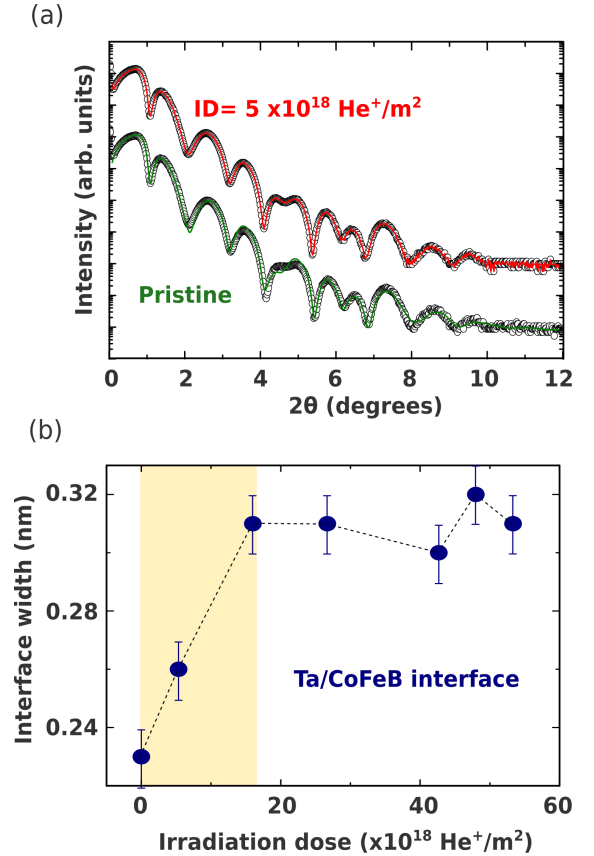
FIG. 3: (a) X-ray reflectivity profiles for a pristine and an irradiated film at ID = 5 \times 10^{18} \text{He}^+/\text{m}^2 , the corresponding model is plotted as solid lines. (b) Width of the Ta/CoFeB interface as a function of the irradiation dose.
