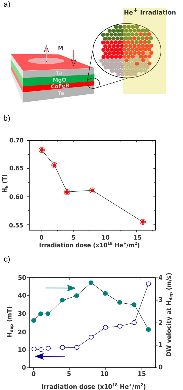
FIG. 1: (a) Sketch depicting the perpendicularly magnetised CoFeB stack and the effect of He + irradiation at the interfaces. (b) Anisotropy field H_k as a function of the irradiation dose. (c) Depinning field H_{dep} (blue circles, left axis) and its corresponding DW velocity v(H_{dep}) (cyan circles, right axis) as a function of irradiation dose.
