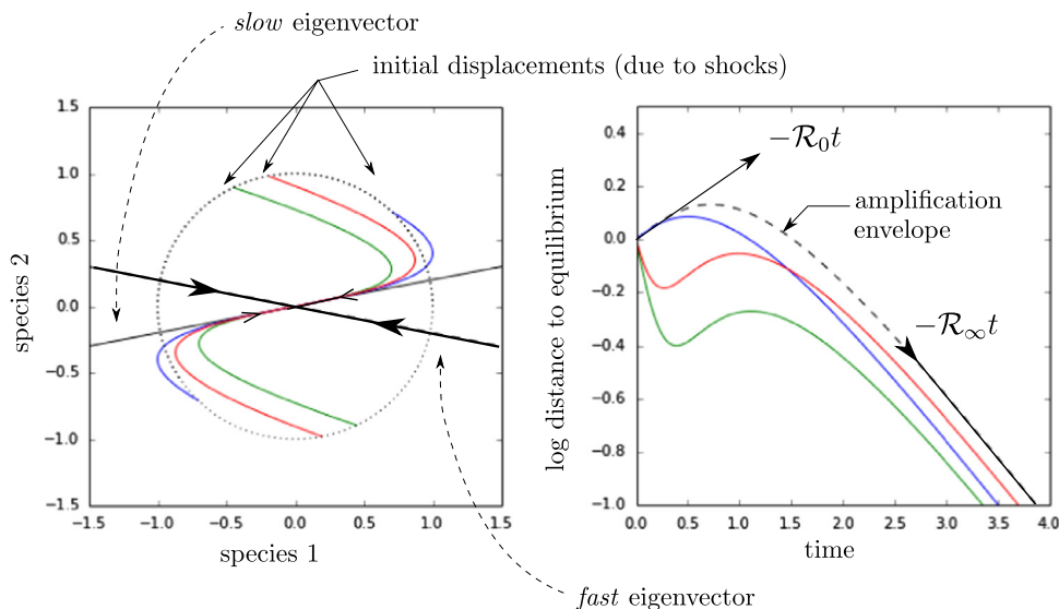
Fig. 2. Definition of asymptotic and initial resilience. The community matrix A = \begin{pmatrix} -1 & 2.5 \\ 0.1 & -1 \end{pmatrix} models a mutualistic community with asymmetric interactions ( A_{12} \neq A_{21} ), near equilibrium. We have \mathcal{R}_\infty = 0.5 and \mathcal{R}_0 = -0.3 , indicating that the system is reactive. We show three trajectories (green, red, blue) starting at unit distance from the equilibrium (and their mirror image). They represent the system response to various normalized shocks. Left panel: plot in phase plane (\mathbf{x}_1, \mathbf{x}_2) , with the eigenvectors represented in black. Right panel: plot of \|\mathbf{x}(t)\| with logarithmic scale on y-axis. The dashed curve represents the amplification envelope, meaning the envelope of the distance to equilibrium of all trajectories starting at distance one. It is computed as the spectral norm of e^{tA} (in log scale on right panel). Asymptotic resilience \mathcal{R}_\infty is the slowest asymptotic rate of return to equilibrium (slope for large time in right panel). Note that a displacement along the fast direction (a non-generic shock) would present a steeper asymptotic slope, corresponding to the real part of the sub-dominant eigenvalue. Initial resilience \mathcal{R}_0 is the slowest initial rate of return to equilibrium (opposite of largest slope at t=0 in right panel). Initial resilience can be negative, as in the example shown here, meaning that there exist trajectories (for example, the blue one) for which the initial displacement is amplified. (For interpretation of the references to color in this figure caption, the reader is referred to the web version of this paper.)
