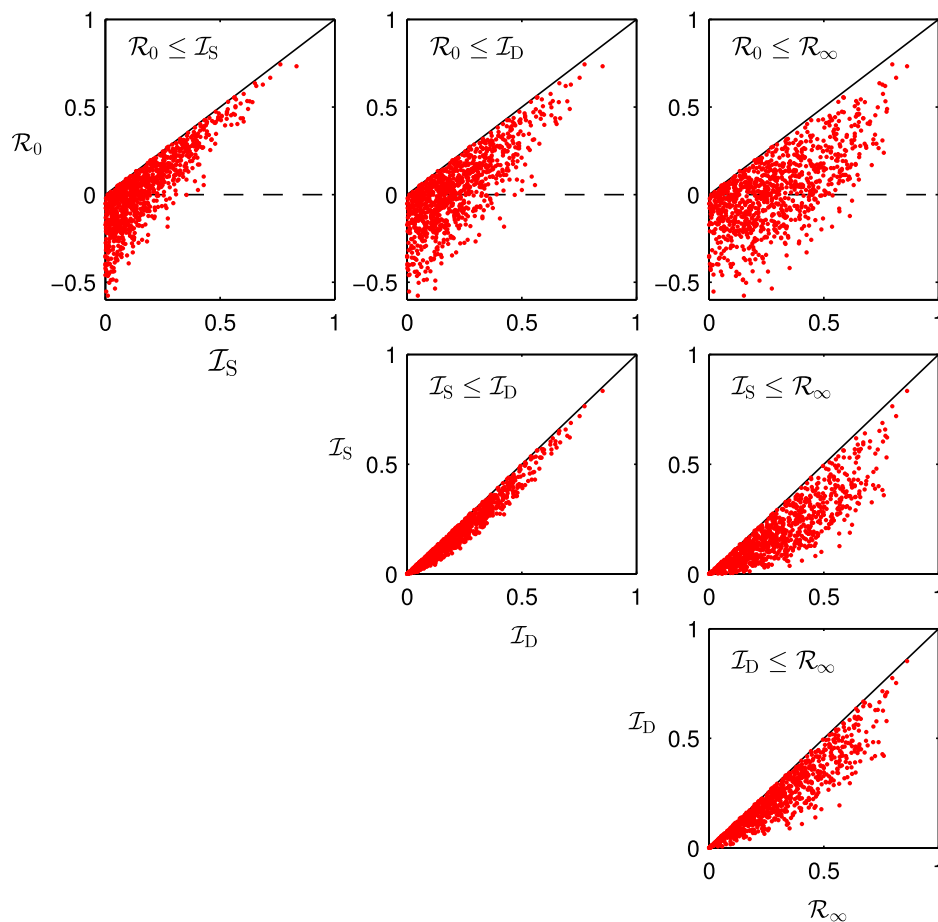
Fig. 5. Illustration of the general stability ordering (12) on random matrices of dimension S=3 . The diagonal elements were drawn from a uniform distribution over [-1, 0] while off-diagonal elements were drawn from a normal distribution of mean 0 and variance 1. With this procedure 63% of the matrices generated were stable. We plotted all four stability measures against each other for 1000 stable matrices (each red dot corresponds to a stable matrix). Dots lying below the full black lines correspond to relatively reactive matrices; dots lying below the dashed black line (top row panels) correspond to reactive matrices. (For interpretation of the references to color in this figure caption, the reader is referred to the web version of this paper.)
