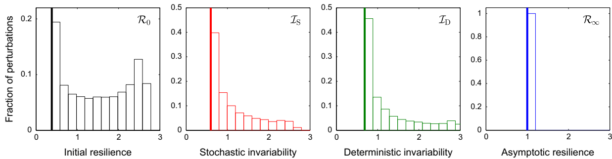
Fig. 7. Worst-case vs generic perturbations. For the community matrix A = \begin{pmatrix} -1 & 2 \\ 0 & -2 \end{pmatrix} , we investigate the system response to random perturbations and compare with the worst-case scenario. In each panel, the vertical thick line represents the intrinsic stability measure, i.e., the system response corresponding to the worst-case scenario, over the defining set of perturbations associated to that measure. The histogram represents the distribution of the system response to a perturbation randomly sampled from the defining set. For resilience measures (left- and rightmost panel), we generated 1000 initial displacements, drawn uniformly on the unit sphere around equilibrium. For stochastic invariability (second panel), we generated 1000 random matrices T of independent Gaussian variables, and constructed white-noise covariance matrices by normalizing \Sigma = TT^T (Wishart distribution). For deterministic invariability (third panel), we generated 1000 random press perturbations (i.e., of frequency \omega = 0 , which is the resonant frequency of this system), uniformly distributed on the sphere. Only asymptotic resilience is generic, as all asymptotic return rates equal \mathcal{R}_\infty . For other measures, the worst-case response can be very different from the response to a particular perturbation.
