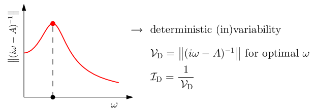
Fig. 4. Definition of intrinsic deterministic invariability. (Top) A periodic perturbation of frequency \omega is applied to the system. In phase space the perturbation defines an ellipse characterized by a complex vector \mathbf{u} . The system response oscillates at the same frequency along an ellipse characterized by the complex vector \mathbf{v} = (i\omega - A)^{-1}\mathbf{u} . The variability of the response is measured as the norm of \mathbf{v} . (Middle) We then look for the maximal response over all input vectors \mathbf{u} , giving the frequency response. We get the frequency response without having to solve an optimization problem, by simply computing the spectral norm of (i\omega - A)^{-1} . (Bottom) We search for the resonant frequency, giving deterministic variability as the maximal frequency response: \mathcal{V}_D = \sup_{\omega} \|(i\omega - A)^{-1}\| . Its inverse is deterministic invariability \mathcal{I}_D .
