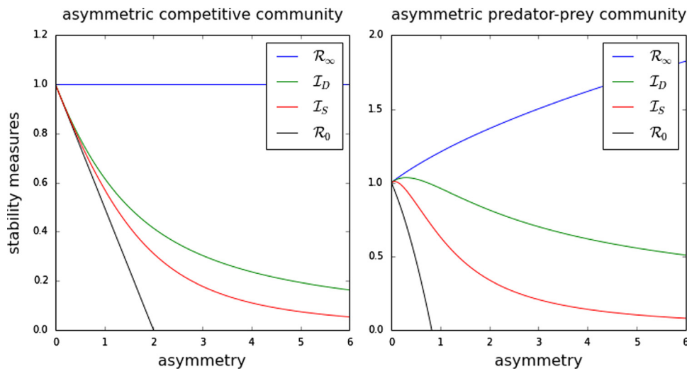
Fig. 6. Branching of stability measures as interaction asymmetry increases. Left panel: the community matrix A = \begin{pmatrix} -1 & -\rho \\ 0 & -1 \end{pmatrix} models the dynamics of two species near equilibrium, with one of them having negative impact on the other. As interaction asymmetry -parametrized by \rho \geq 0 - grows, asymptotic resilience remains unchanged while the other measures drop. At \rho = 6 asymptotic resilience is one order of magnitude larger than stochastic invariability. Right panel: the matrix A = \begin{pmatrix} -1 & -(1+\rho^2) \\ 1 & -\sqrt{1+\rho} \end{pmatrix} models a consumer-resource system near equilibrium, with the consumer depleting, for a fixed benefit, a growing amount of resource. As asymmetry grows, asymptotic resilience increases while other measures show a loss of stability. We observe that in both examples, the system becomes reactive ( \mathcal{R}_0 < 0 ) at low asymmetry.
