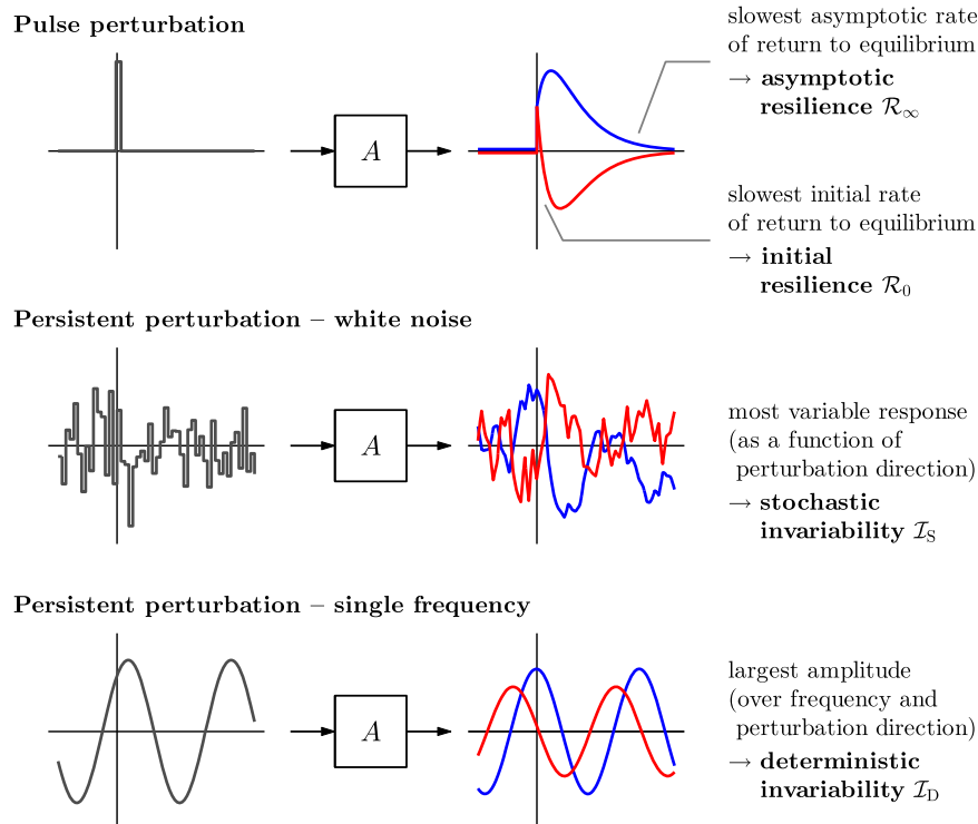
Fig. 1. Four measures of ecological stability. Stability can be quantified by applying a perturbation (left graphs) to a system (here represented by community matrix A ) and measuring its response (right graphs; curves can be interpreted as biomass changes of two species through time). Each stability measure we consider corresponds to the worst-case system response for a specific class of perturbations. Asymptotic resilience \mathcal{R}_\infty is the slowest asymptotic rate of return to equilibrium after a pulse perturbation. Initial resilience \mathcal{R}_0 is the slowest initial recovery rate. Intrinsic stochastic invariability \mathcal{I}_S is inversely proportional to the variance of the maximal response to white-noise perturbations. Intrinsic deterministic invariability \mathcal{I}_D is the inverse of the amplitude of the maximal response to single-frequency perturbations. In this paper we show that these four measures are comparable, despite the different classes of perturbations considered.
