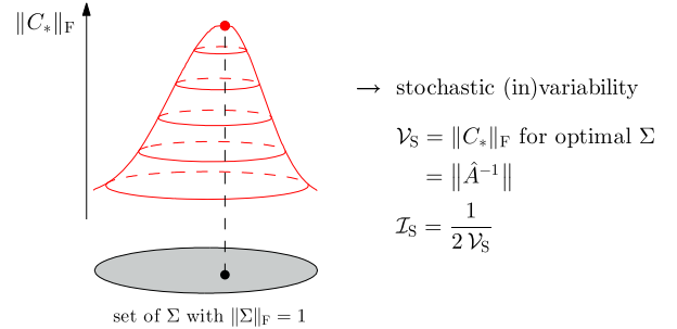
Fig. 3. Definition of intrinsic stochastic invariability. (Top) White noise is applied to the system. It can be seen as a continuous successions of normally distributed (infinitesimal) shocks, characterized by a covariance matrix \Sigma . The response of the system to white noise is continuous, and normally distributed in phase plane, with covariance matrix C_* = -\hat{A}^{-1}(\Sigma) . The variability of the response is measured as the Frobenius norm of this matrix. (Bottom) To get an intrinsic measure, we look for the worst-case scenario, i.e., the input matrix \Sigma generating the maximal variability. However, we show that the maximal response can be computed without having to solve an optimization problem. To get stochastic variability \nu_S , it suffices to compute the spectral norm of \hat{A}^{-1} . Stochastic invariability \mathcal{I}_S is then defined as half of the inverse of \nu_S .
